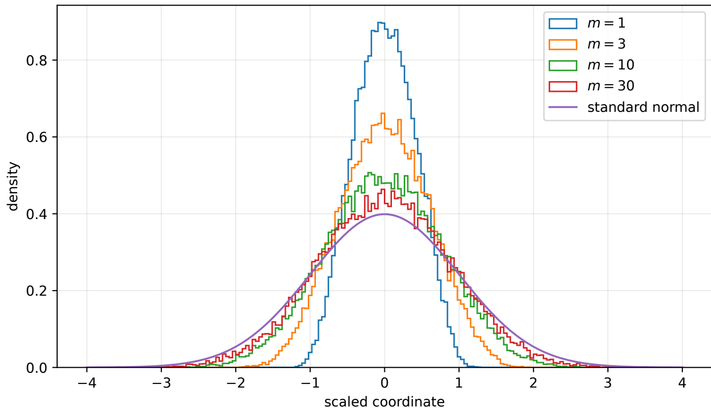
Occupancy-sampled densities of \sqrt{2m} \gamma^{[m]}
