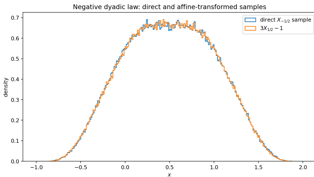
Figure 39: Independent simulations of X_{-1/2} and 3X_{1/2} - 1 . The visual agreement supplements the exact digit-reflection coupling in table 21 .
