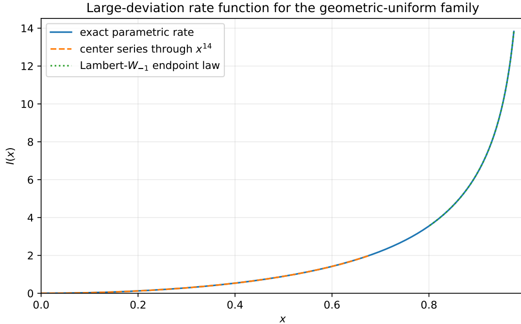
Figure 45: The exact parametric rate I(x) , its rational center expansion, and the Lambert- W_{-1} boundary approximation. The latter is already visually indistinguishable from the exact curve for x \gtrsim 0.8 .
