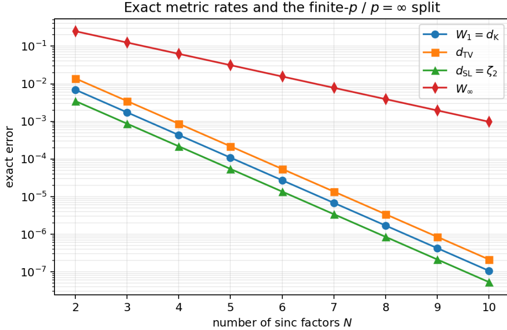
Figure 16: The finite metrics have exact 4^{-N} rates, whereas W_\infty has exact rate 2^{-N} . This is the first indication of the finite- p/p = \infty crossover.
