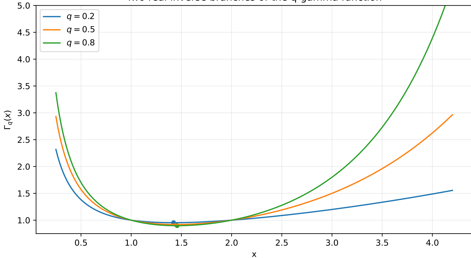
Two real inverse branches of the q-gamma function
