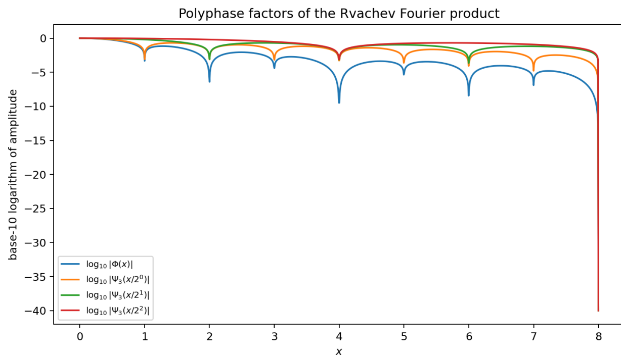
Figure 5: For r = 3 , the logarithmic magnitude of the full Fourier image and its three sparse factors. At each integer zero the component multiplicities add to the multiplicity of \Phi . The graph clips the logarithm near zeros; the product identity itself was checked at high precision away from and near the zero lattice.
