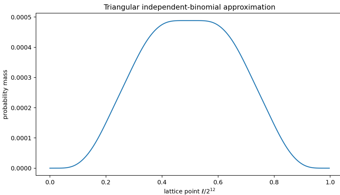
Figure 18: The positive mass distribution encoded by P_{12} . Its broad, nearly flat central region is a finite-layer effect quite different from a single binomial law.
