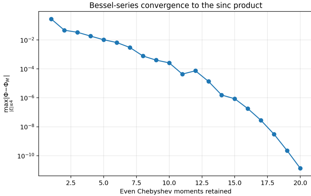
Figure 12: Maximum error on |\xi| \leq 4 of the first M even-order terms in (601), measured against a 90-factor sinc product. At M = 20 , the recorded maximum is approximately 1.35 \times 10^{-11} .
