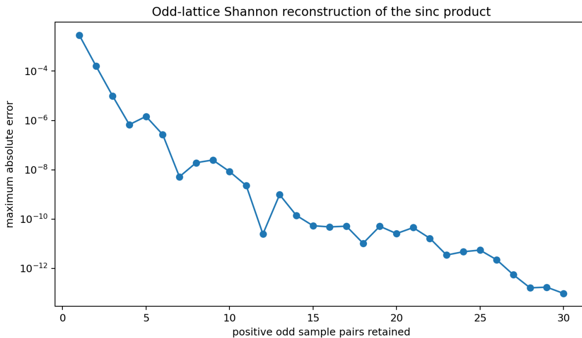
Figure 17: Maximum residual of the odd-sample cardinal formula at two real and one complex test point. The small nonmonotonic ripples reflect cancellation; the envelope decreases superalgebraically.
