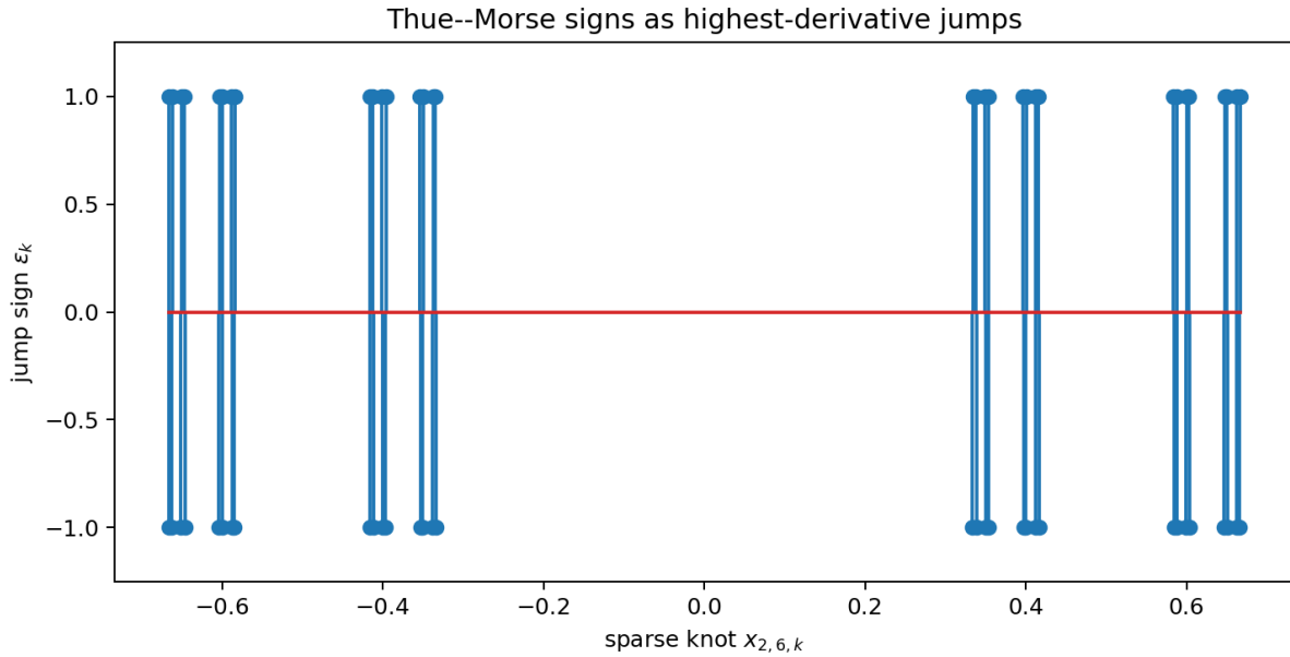
Figure 4: The distribution q^{\binom{N}{2}} D^N g_{r,N} for a finite sparse spline. Reading its signed atoms from left to right gives the ordinary Thue–Morse word because the spatial bit-reversal leaves binary parity unchanged. The plotted example is generated by the accompanying script.
