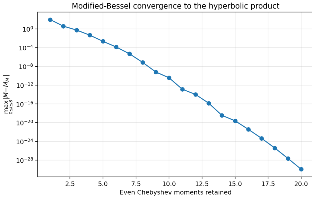
Figure 13: Maximum error on 0 \leq t \leq 8 of the first M even-order terms in (606), measured against a 90-factor hyperbolic product. At M = 20 , the recorded maximum is approximately 1.14 \times 10^{-30} .
