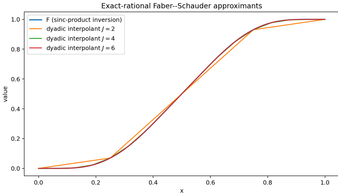
Figure 15: The exact-rational dyadic interpolants are the Faber partial sums. The level-6 curve is already visually indistinguishable from the independent sinc-product reconstruction on most of the interval.
