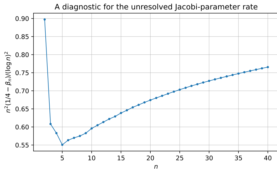
Figure 7: The diagnostic quantity n^2(1/4 - \beta_n)/(\log n)^2 . The range n \leq 40 is evidence, not an asymptotic proof.
