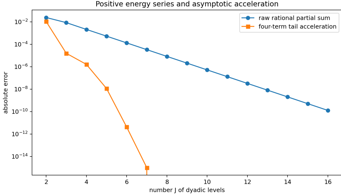
Figure 16: Raw positive rational partial sums converge geometrically. Using four terms of the all-orders tail expansion removes several additional powers of 4^{-J} . Values below machine precision relative to the numerical reference are omitted automatically from the logarithmic plot.
