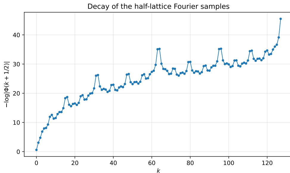
Figure 8: The half-lattice samples decay faster than every power, while their signs are the signed Thue–Morse word. The local irregularity reflects the binary orbit structure.
