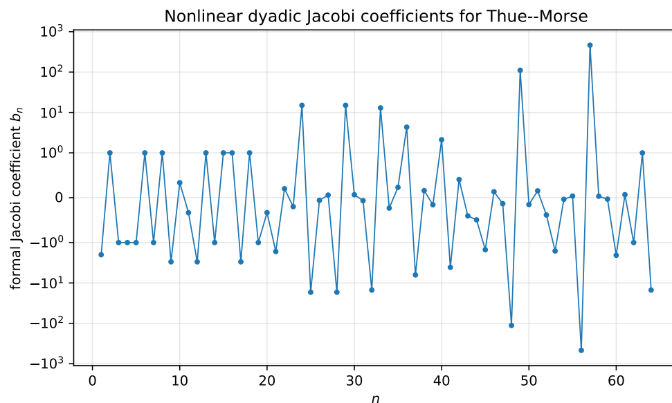
Figure 10: The indefinite formal Jacobi coefficients b_n , shown on a symmetric logarithmic scale. Their nonlinear dyadic recursion creates simultaneous very large and very small rational values.
