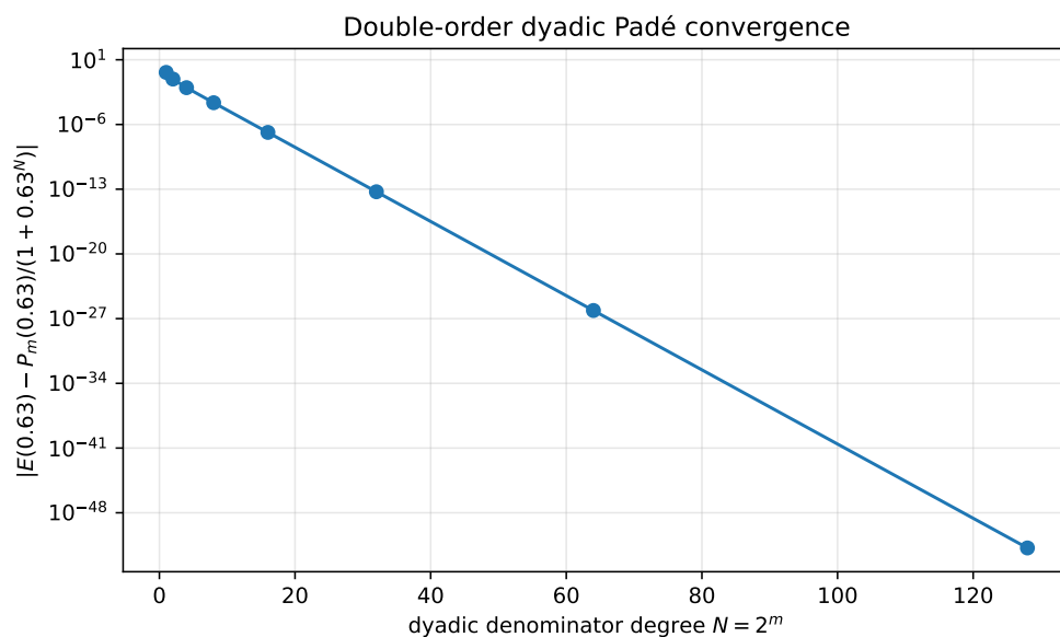
Figure 11: Error of the explicit dyadic Padé approximant at z = 0.63 . The order doubles with each dyadic level, as proved in Theorem T.1.
