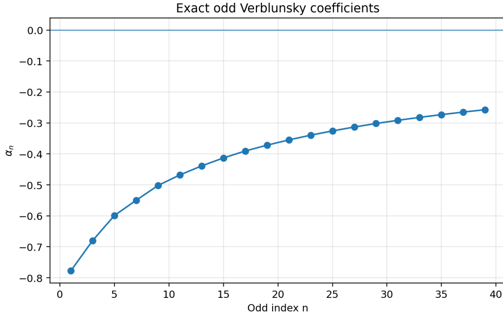
Figure 14: The first twenty exact odd Verblunsky coefficients. All even coefficients vanish. The displayed odd values are negative and increase toward zero, motivating theorem M.1 ; Rakhmanov’s theorem proves convergence to zero but not the observed sign and monotonicity.
