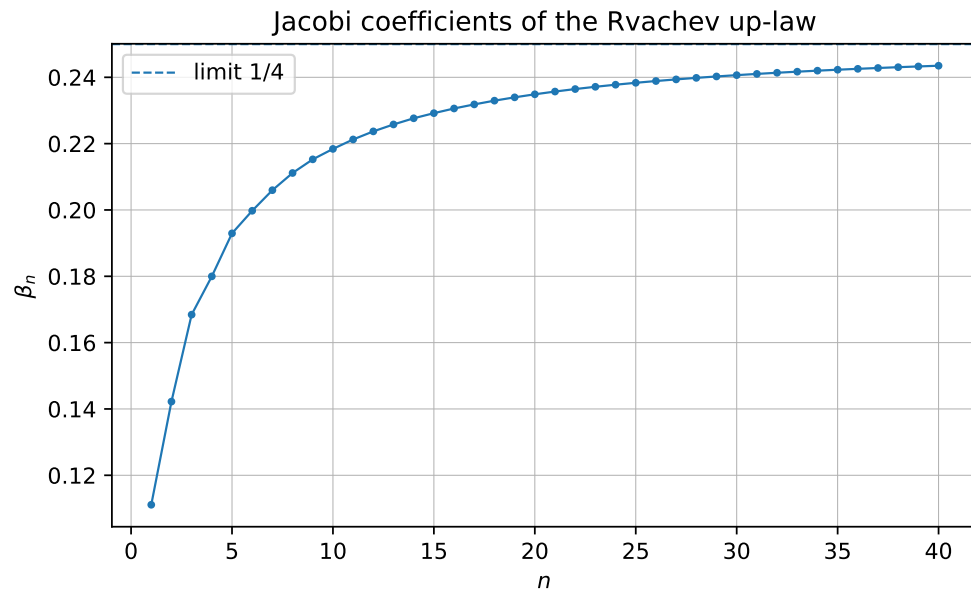
Figure 6: Exact Jacobi coefficients converted to decimals. The dashed line is the proved limit 1/4 .
