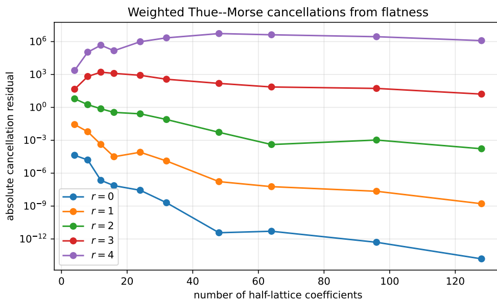
Figure 9: Truncation residuals in the spectral Prouhet identities (482). Higher powers initially amplify the tail before the super-polynomial Fourier decay dominates.
