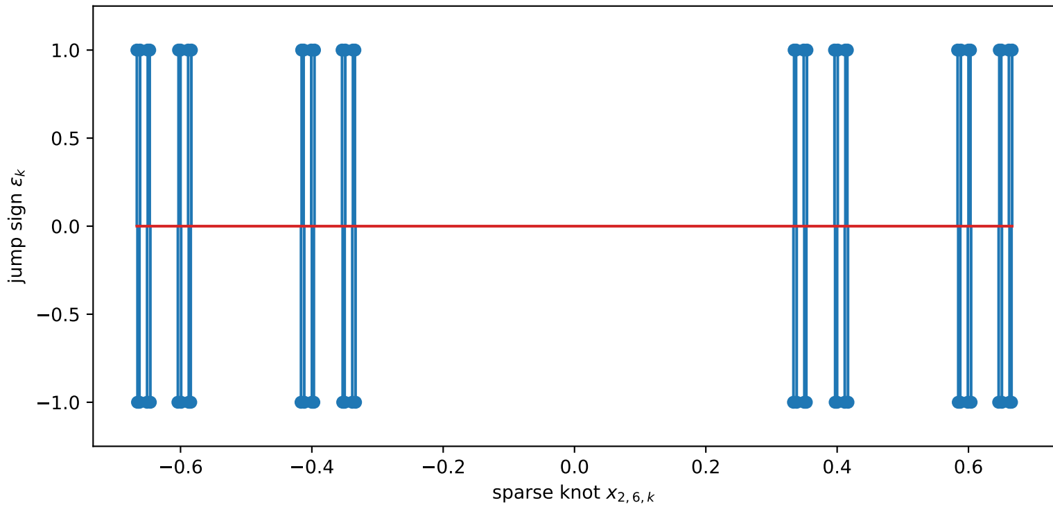
Thue--Morse signs as highest-derivative jumps
