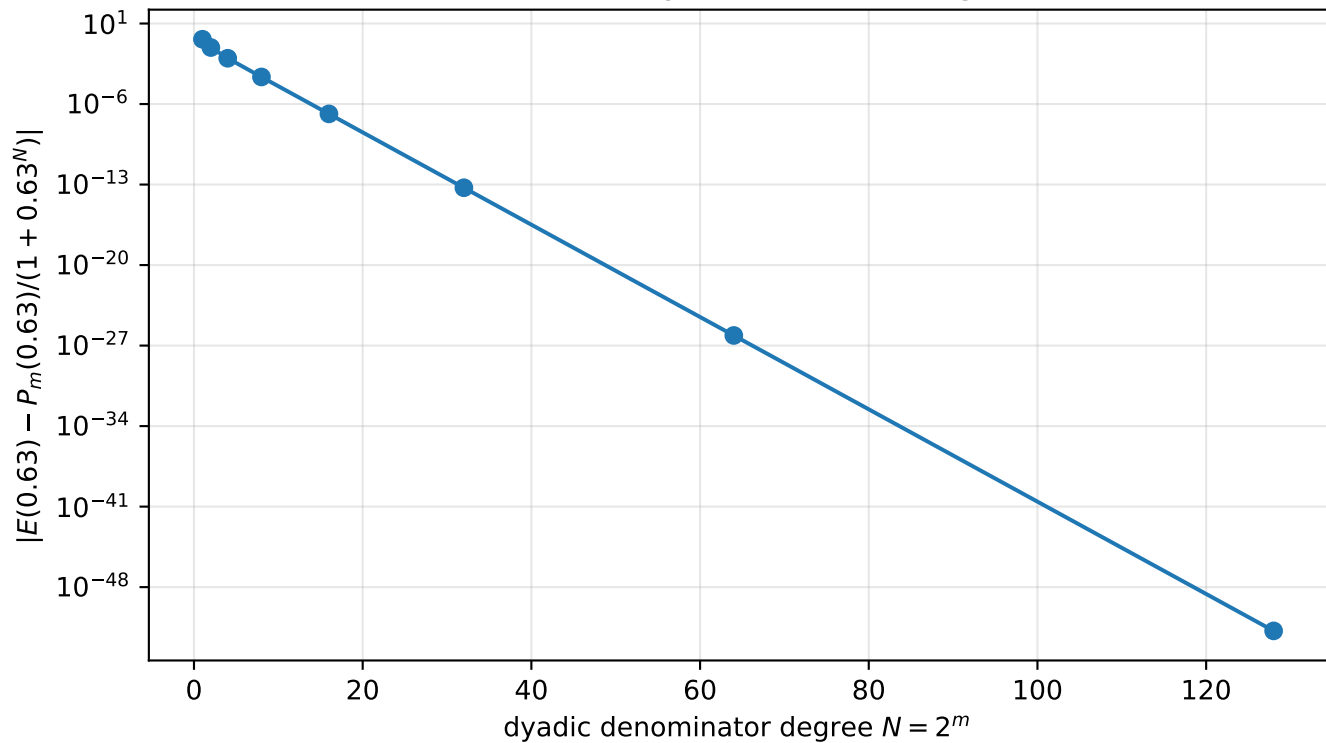
Double-order dyadic Padé convergence
