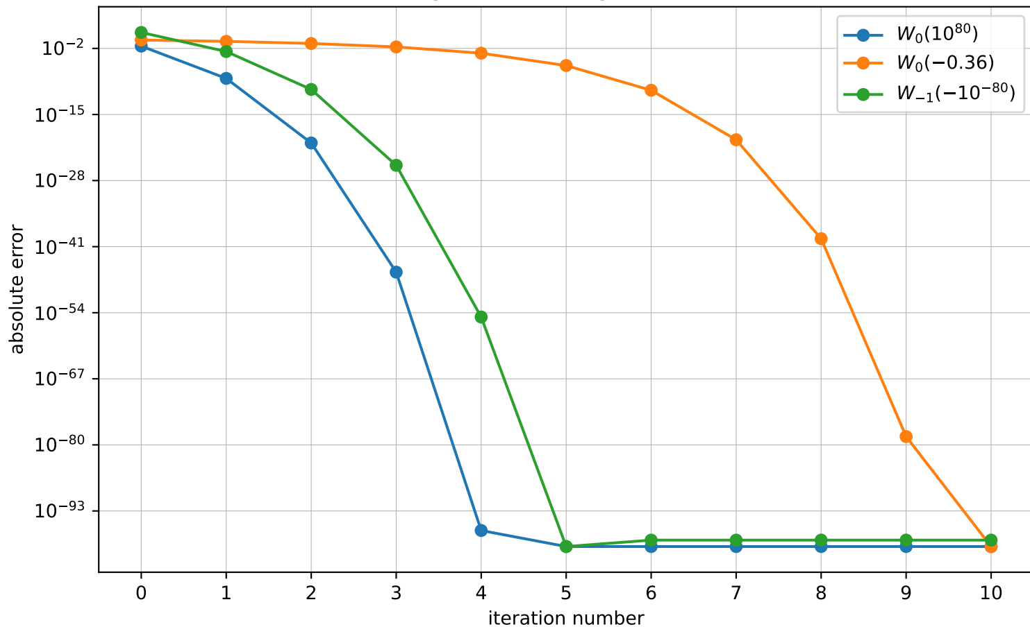
Quadratic convergence of the logarithmic Newton iteration
