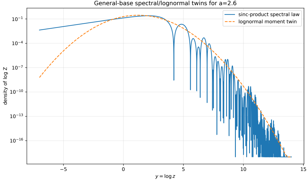
Figure 21: The spectral density of Z_a against its lognormal moment twin for representative bases. The two densities share every moment (12.1) yet differ on an interval (corollary 12.2).
