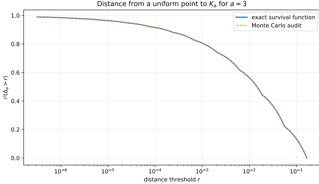
Figure 27: The distance \Delta to the nonanalytic set at a = 3 : empirical law of a uniform sample against the exact tube-formula distribution (15.15).
