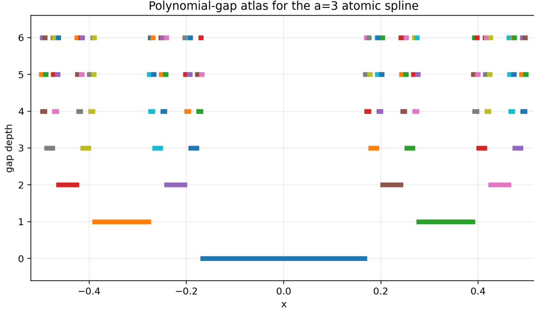
Figure 24: The first seven levels of the gap decomposition for a = 3 . The depth r gaps are the intervals on which the local polynomial degree is exactly r . Their union has full measure in the support [-1/2, 1/2] .
