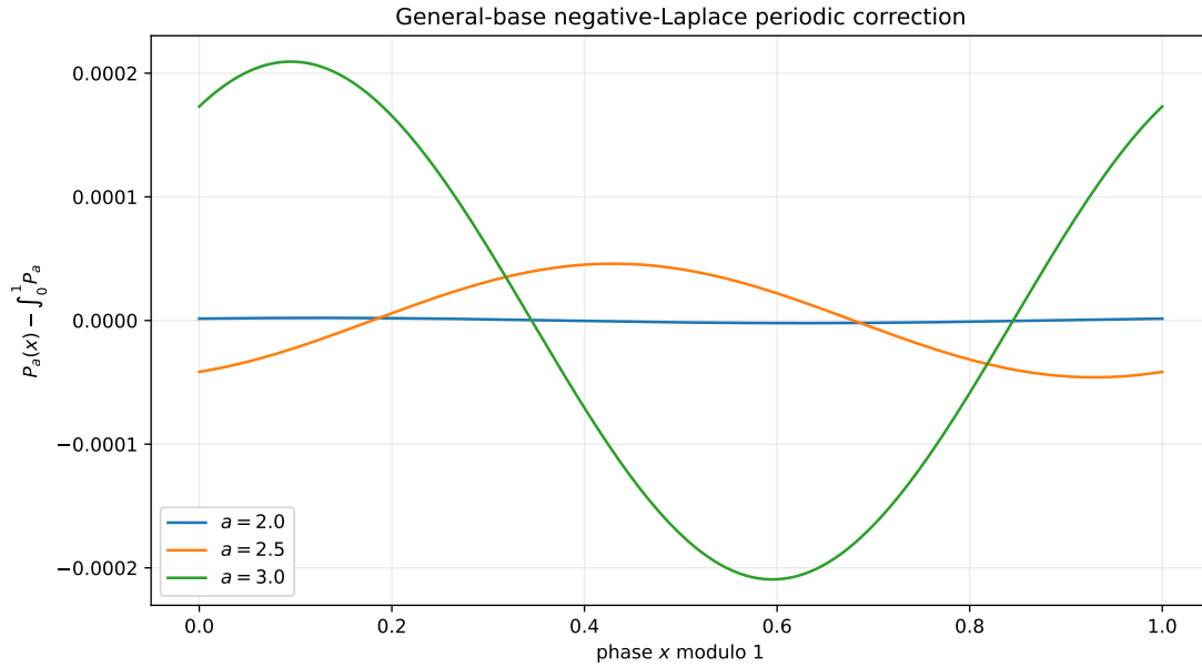
Figure 32: Centered periodic corrections \Psi_a = P_a - \bar{P}_a for several bases. The dyadic oscillation has amplitude of order 10^{-6} ; the amplitude grows substantially with the base, following the mode formula (21.17).
