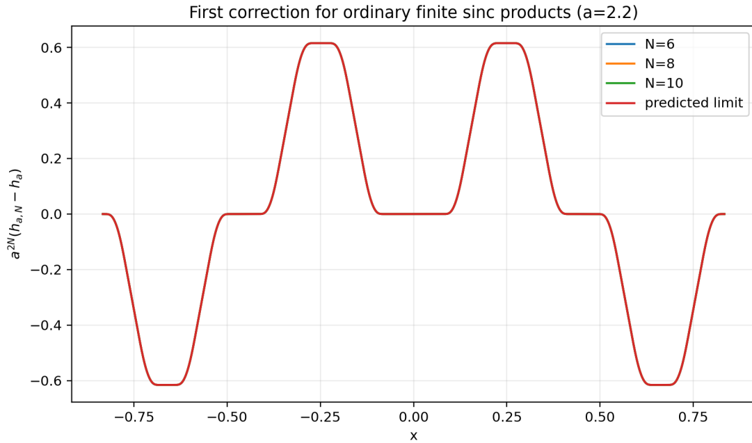
Figure 29: For a = 2.2 , the scaled errors a^{2N}(h_{a,N} - h_a) for N = 6, 8, 10 are visually indistinguishable from -h_a''/[6(a^2 - 1)] . The computation uses FFT inversion of the explicit products, not random sampling.
