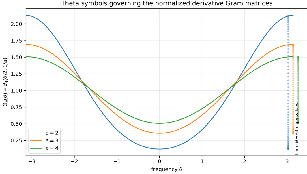
Figure 23: The exact Toeplitz symbols \Theta_a for a = 2, 3, 4 (proposition 13.6). The vertical point clouds at the right are the eigenvalues of the corresponding 64 \times 64 Gram sections; they lie inside, and increasingly fill, the optimal theta intervals [A_a, B_a] of (13.6).
