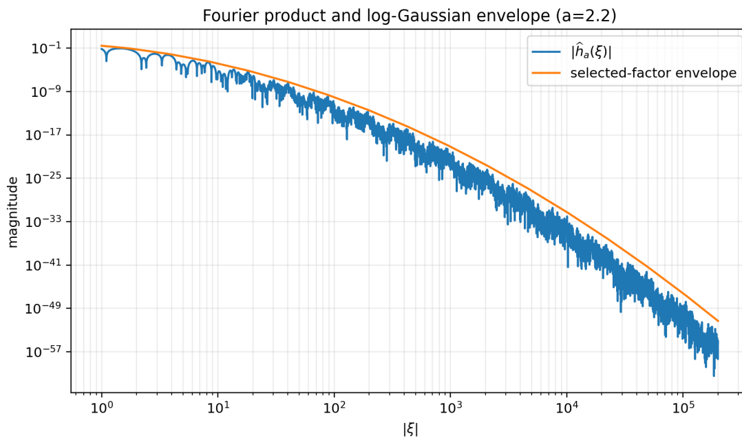
Figure 28: The Fourier product for a = 2.2 and the selected-factor bound (17.1). The oscillatory zeros sit well below the envelope, while the quadratic decay in \log |\xi| is clearly visible.
