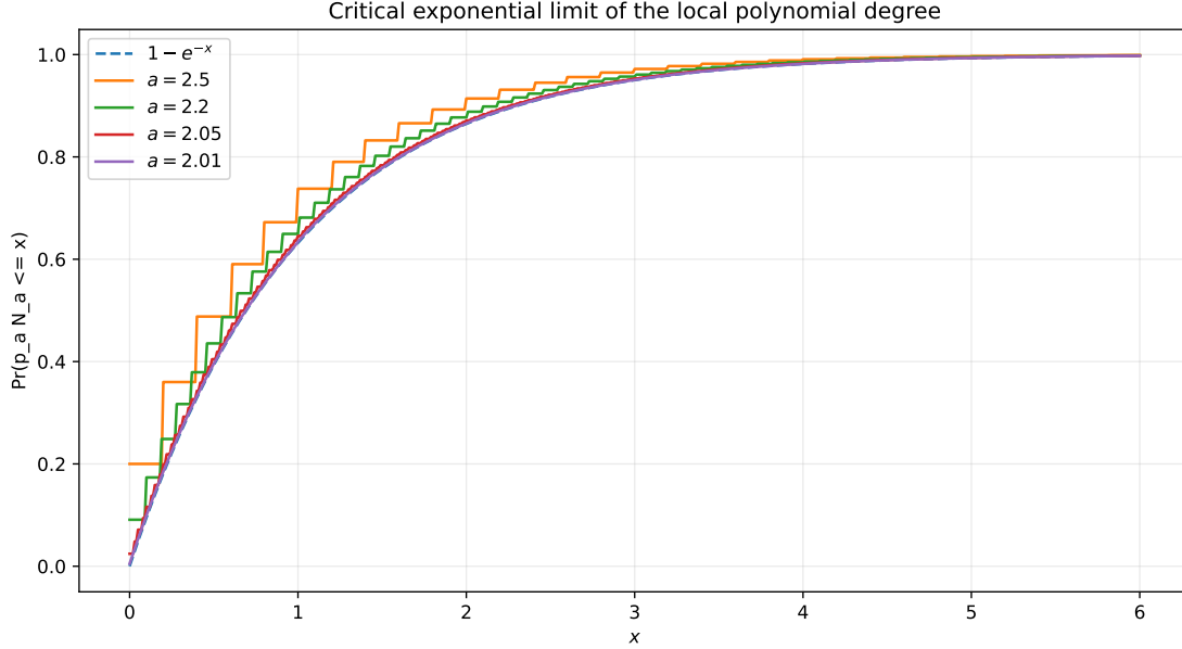
Figure 26: Distribution functions of p_a N_a approaching 1 - e^{-x} as a \downarrow 2 (theorem 15.3).
