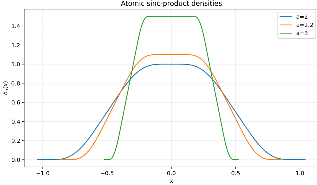
Figure 30: Profiles of h_a at the critical point a = 2 and in the separated regime. The central plateau has height a/2 and half-width (a - 2)/(a(a - 1)) for a > 2 ; it collapses to the single maximum of up at a = 2 .
