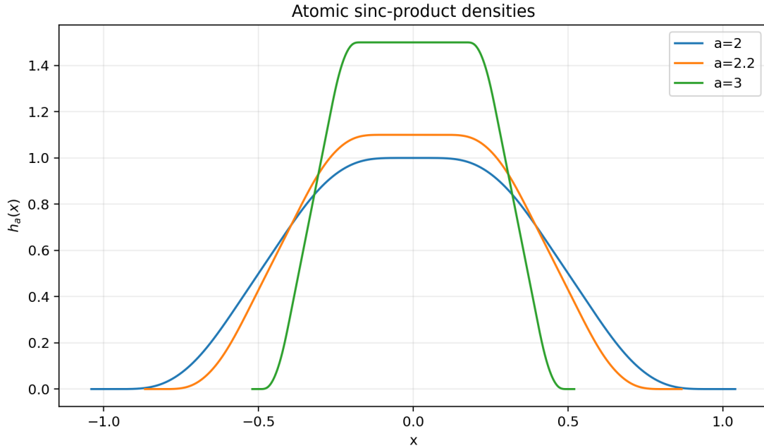
Figure 27: Profiles of h_a at the critical point a = 2 and in the separated regime. The central plateau has height a/2 and half-width (a-2)/(a(a-1)) for a > 2 ; it collapses to the single maximum of up at a = 2 .
