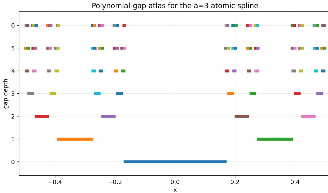
Figure 21: The first seven levels of the gap decomposition for a = 3 . The depth r gaps are the intervals on which the local polynomial degree is exactly r . Their union has full measure in the support [-1/2, 1/2] .
