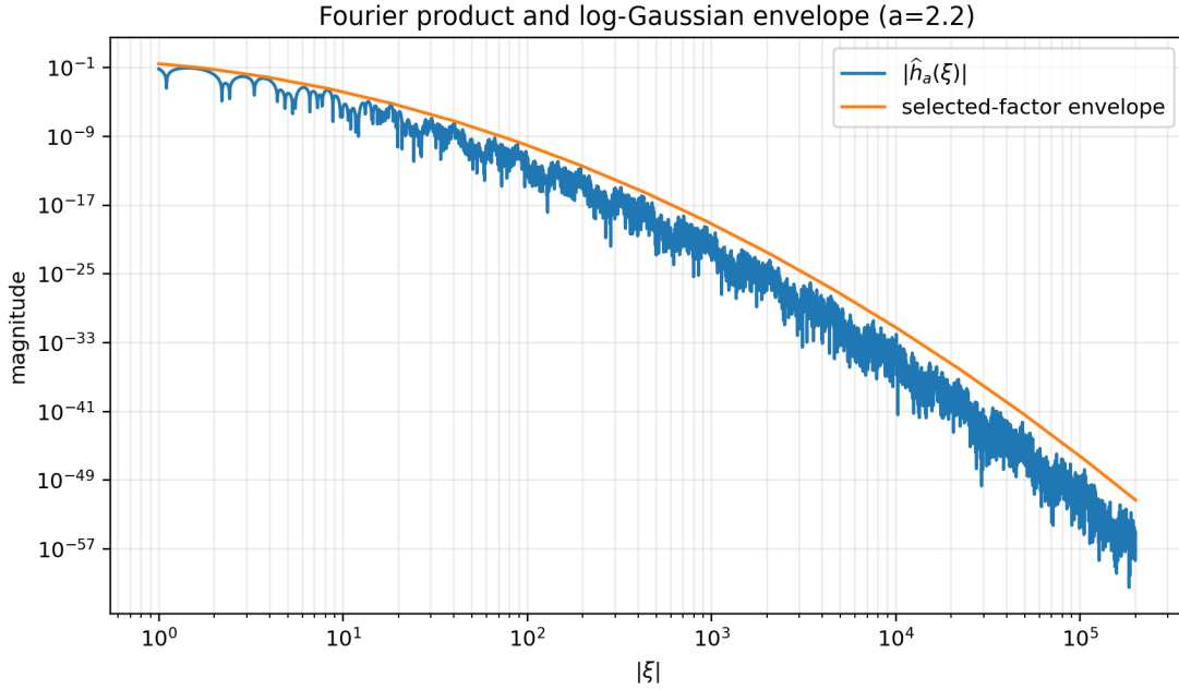
Figure 25: The Fourier product for a = 2.2 and the selected-factor bound (16.1). The oscillatory zeros sit well below the envelope, while the quadratic decay in \log |\xi| is clearly visible.
