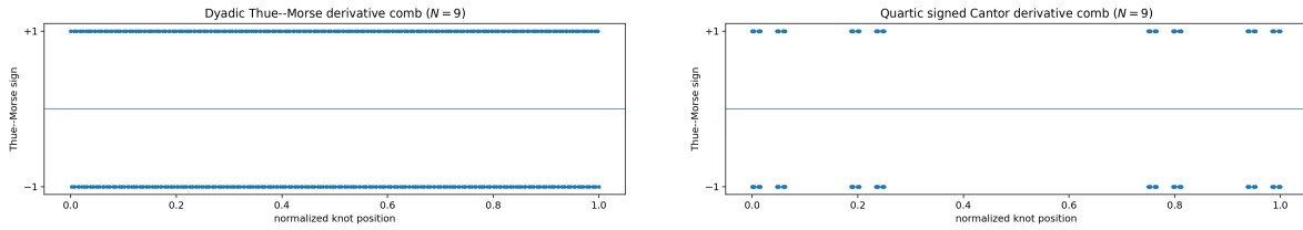
Figure 31: Signed derivative combs at level N = 9 (ordinate: Thue–Morse sign). Left, q = 1/2 : a full dyadic grid. Right, q = 1/4 : base-four digits \{0, 1\} already displaying the dimension- 1/2 Cantor geometry of (12.2).
