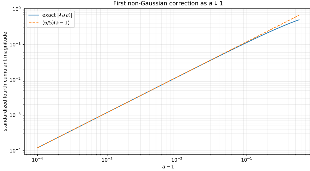
Figure 28: The exact standardized fourth cumulant (19.3) and its first asymptotic term as a \downarrow 1 .
