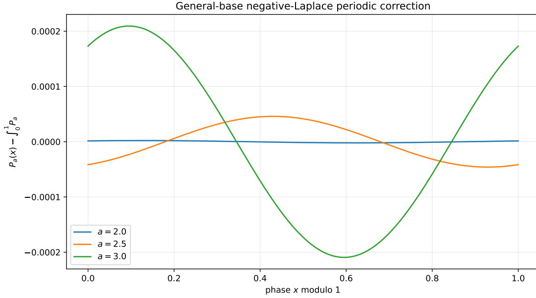
Figure 29: Centered periodic corrections \Psi_a = P_a - \bar{P}_a for several bases. The dyadic oscillation has amplitude of order 10^{-6} ; the amplitude grows substantially with the base, following the mode formula (20.17).
