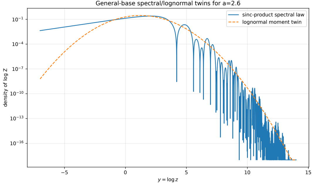
Figure 20: The spectral density of Z_a against its lognormal moment twin for representative bases. The two densities share every moment (12.1) yet differ on an interval (corollary 12.2).
