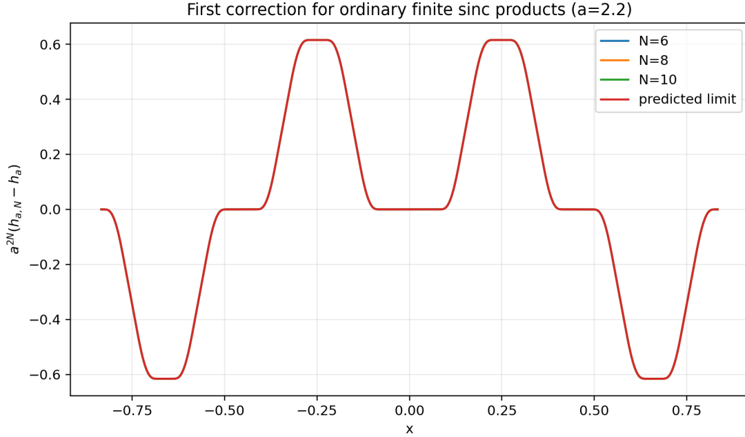
Figure 26: For a = 2.2 , the scaled errors a^{2N}(h_{a,N} - h_a) for N = 6, 8, 10 are visually indistinguishable from -h_a''/[6(a^2 - 1)] . The computation uses FFT inversion of the explicit products, not random sampling.
