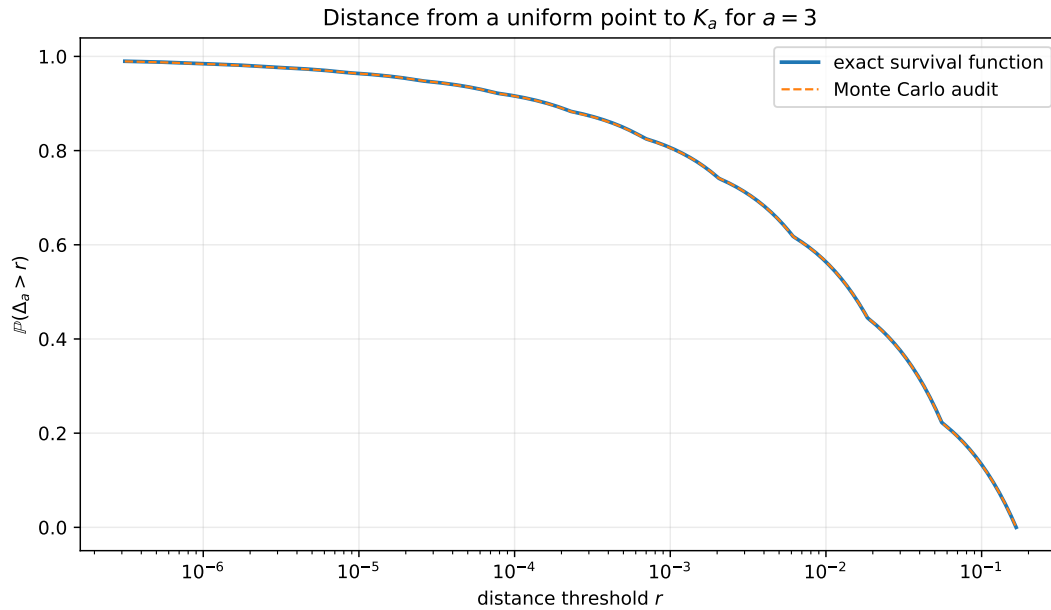
Figure 24: The distance \Delta to the nonanalytic set at a = 3 : empirical law of a uniform sample against the exact tube-formula distribution (14.15).
