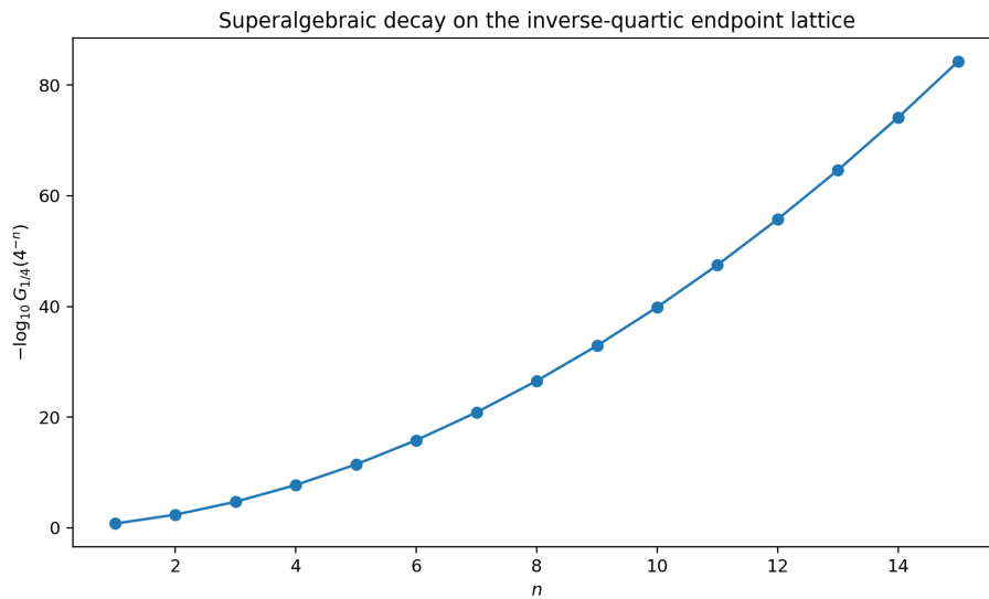
Figure 32: Exact inverse-quartic lattice values (14.3) on a logarithmic ordinate. The quadratic growth of -\log G_{1/4}(4^{-n}) is the discrete shadow of the two-term endpoint law of theorem 15.1.
