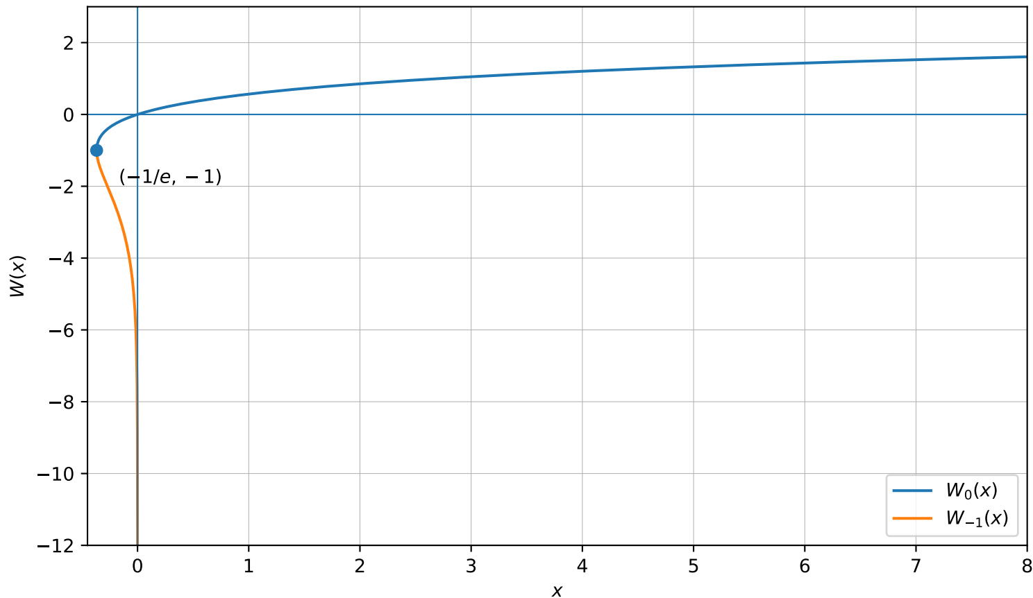
The two real branches of the Lambert W function
