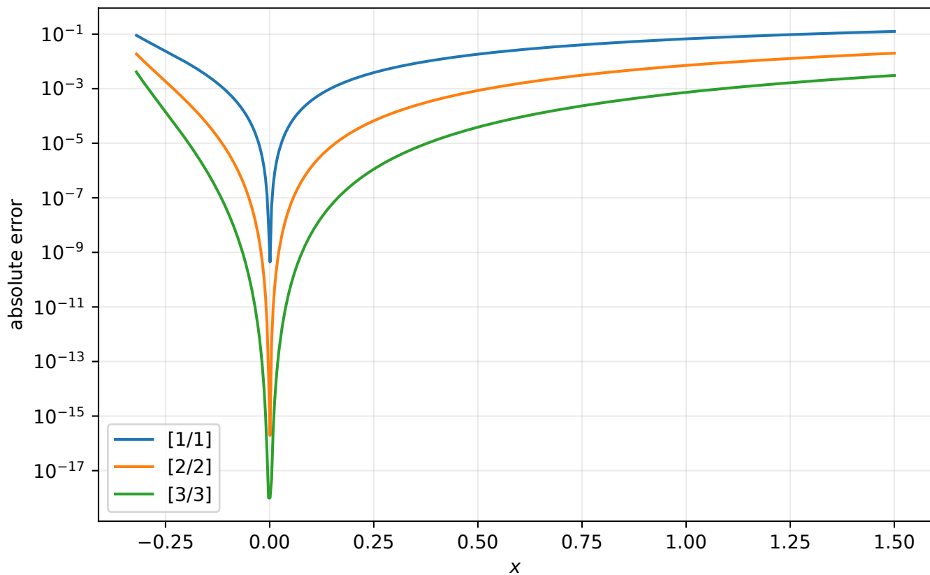
Pade approximants to W_0 about the origin
