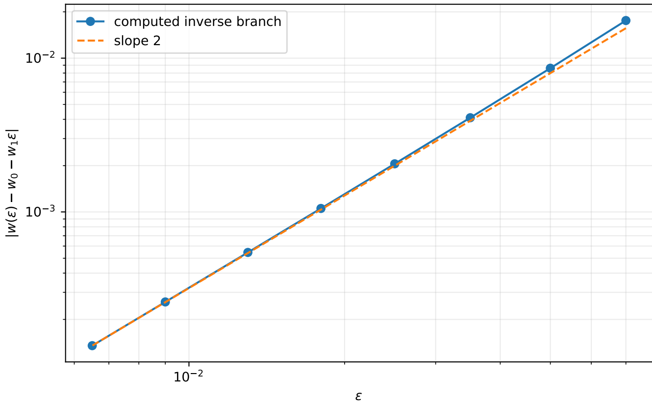
Inverse cyclotomic frequency branch, m=4
