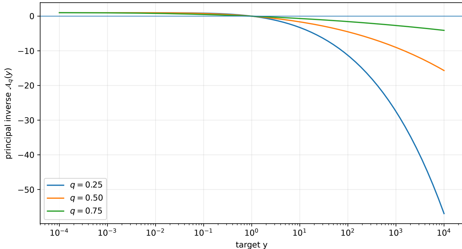
Principal real inverse of the infinite q-Pochhammer product
