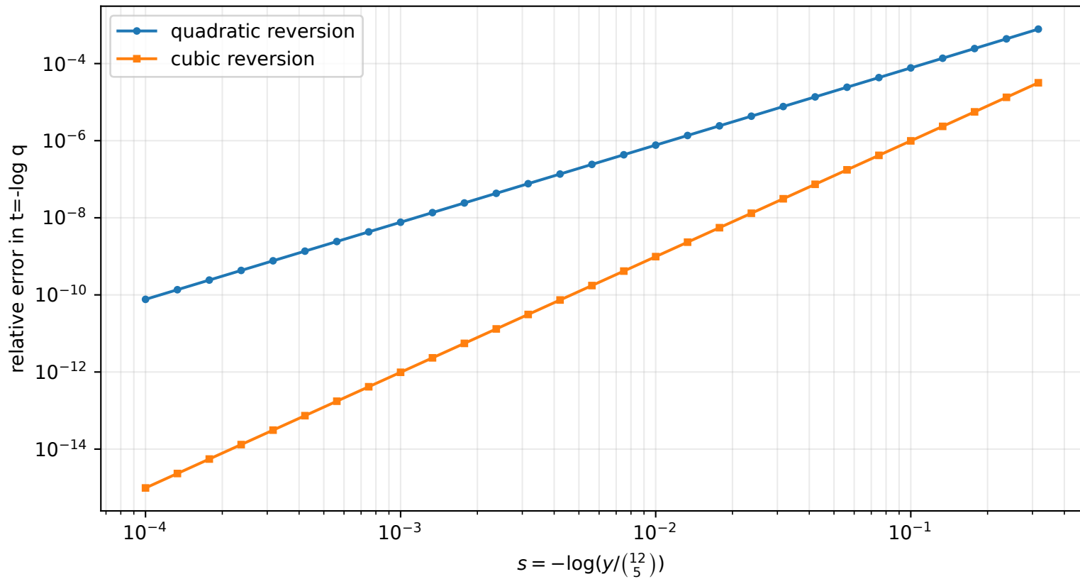
Near- q=1 inversion of a Gaussian coefficient
