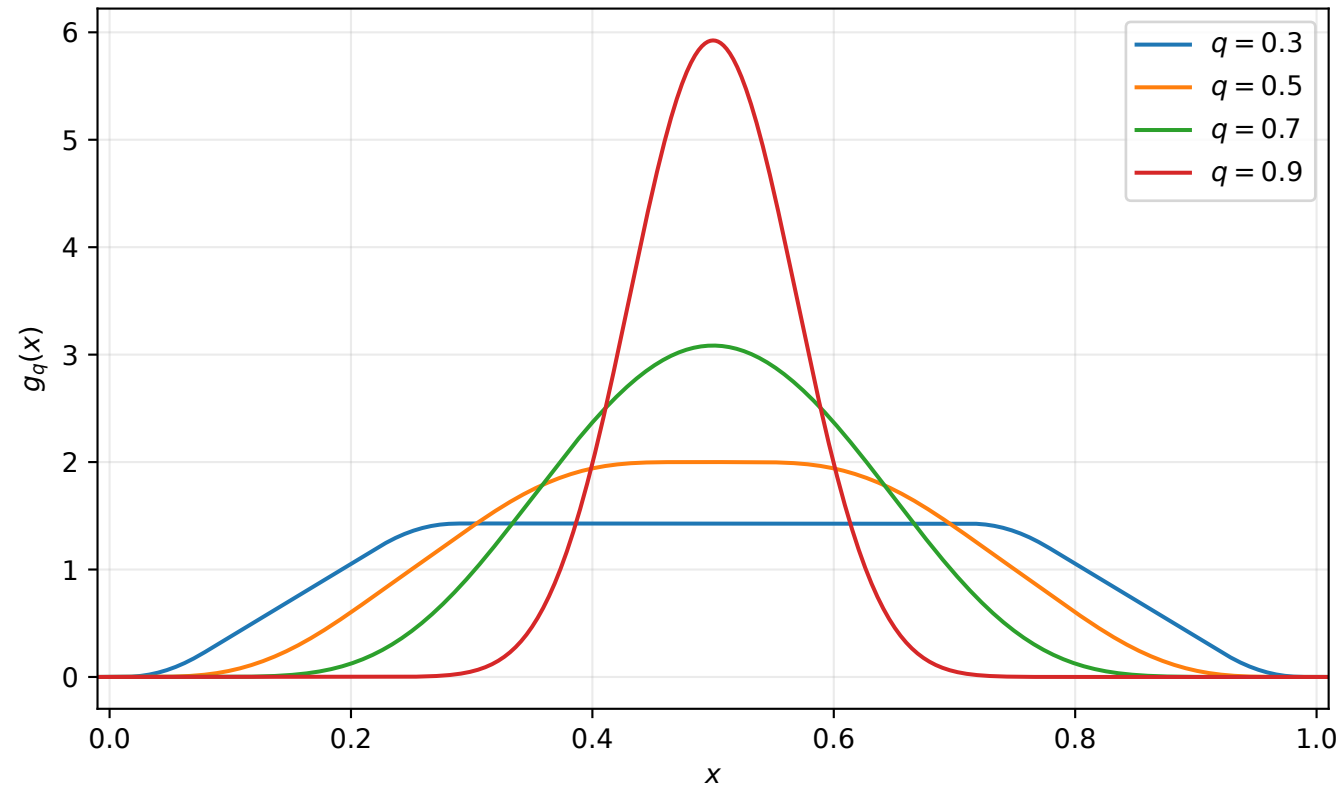
Geometric-uniform densities
