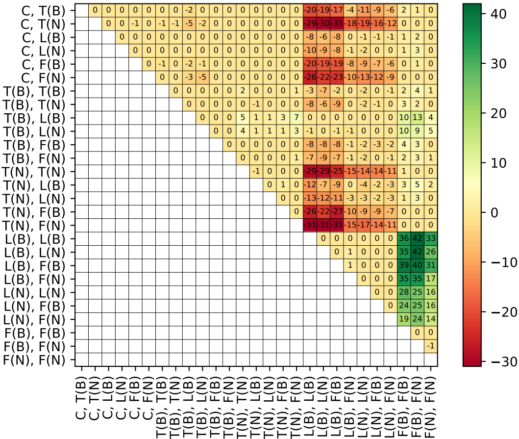
Population size 200, replacement "Sort"
