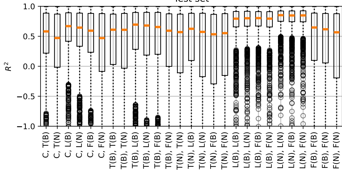
Test set
