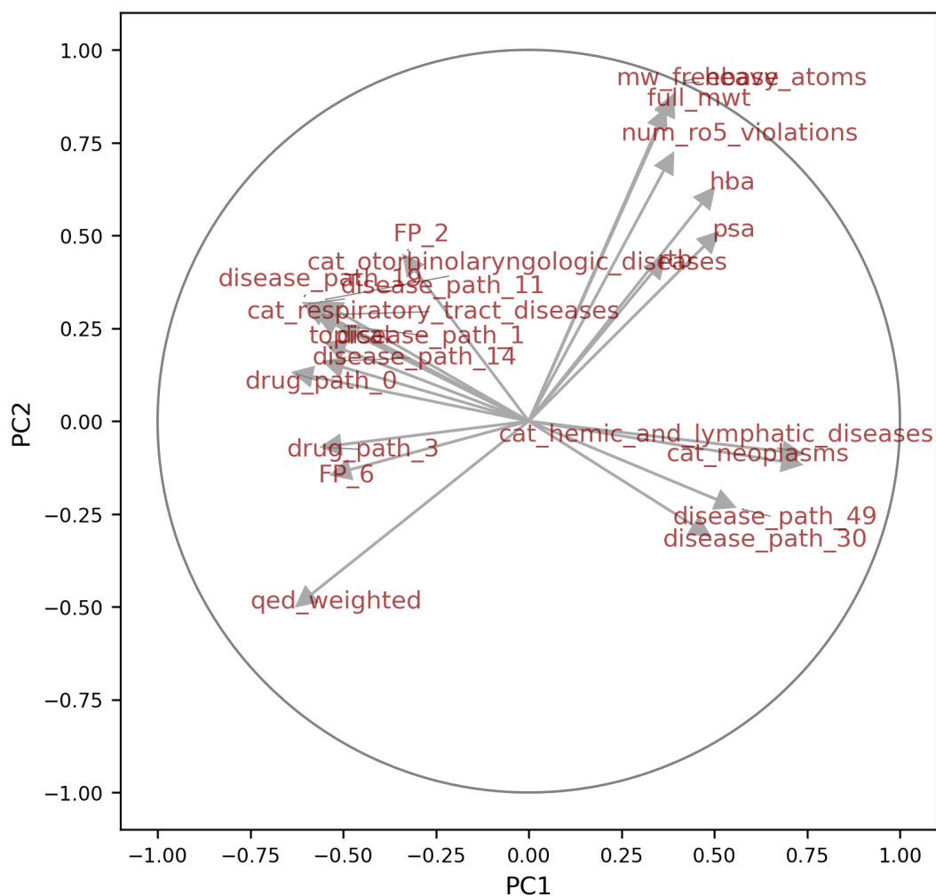
Figure A11: PCA correlation circle showing feature contributions to the first two principal components. Only arrows with length above 0.5 are shown.
