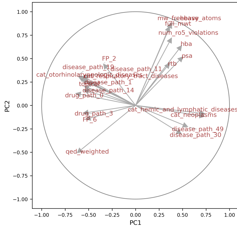
Figure 6: PCA correlation circle.
