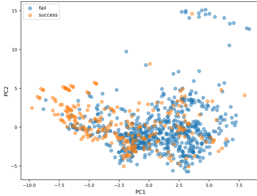
Figure 5: PCA scatter plot.
