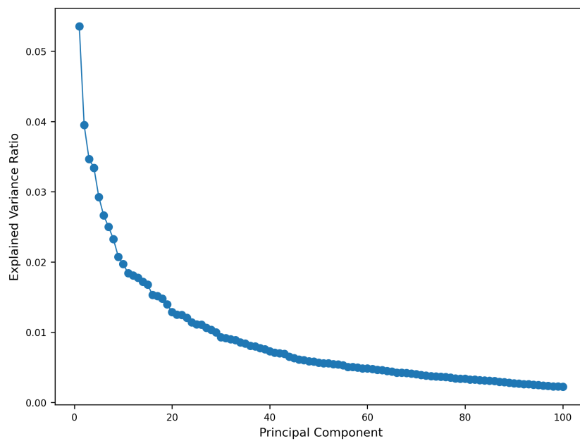
Figure 4: Scree plot of PCA on merged data.
