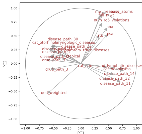
Figure 8: PCA correlation circle showing feature contributions to the first two principal components. Only arrows with length above 0.5 are shown.
