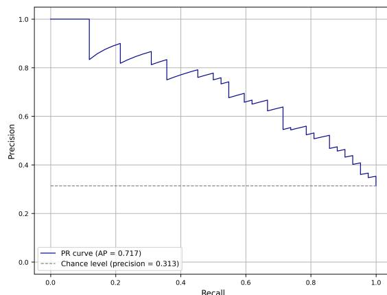
Figure 10: Precision-recall curve for XGBoost on the test dataset.
