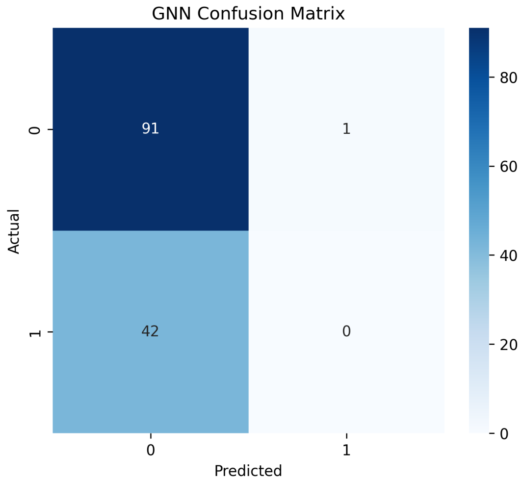
Figure A13: Confusion matrix for Heterogenous GNN on the test dataset.
