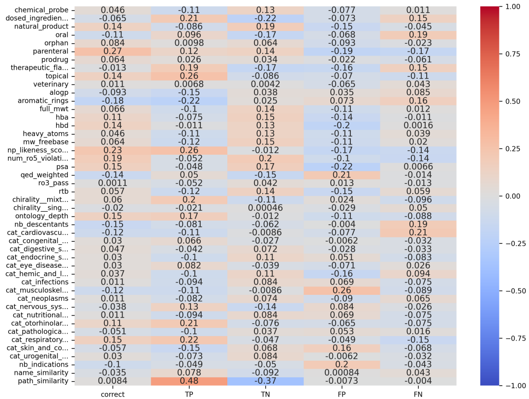
Figure A15: Correlation heatmap of XGBoost test classification results with predictors.
