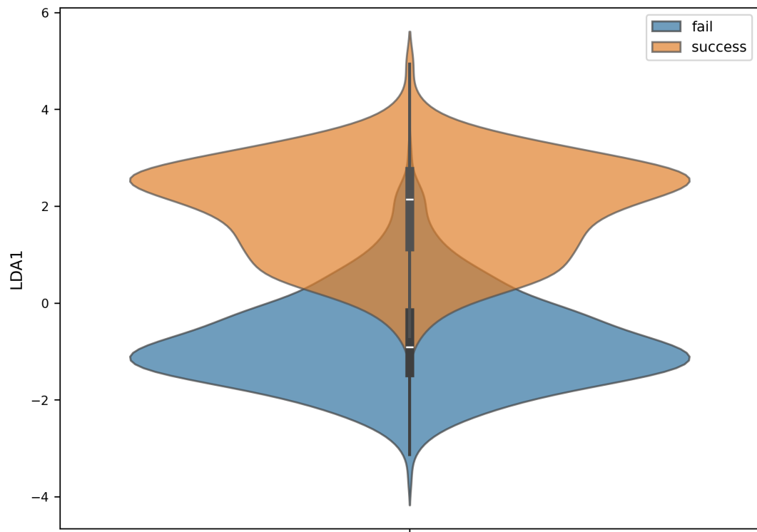
Figure A10: Linear Discriminant Analysis (LDA) projection highlighting class separation.
