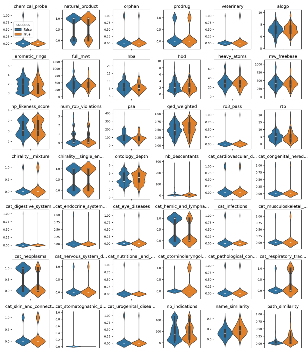
Figure A3: Feature distributions by success label.
