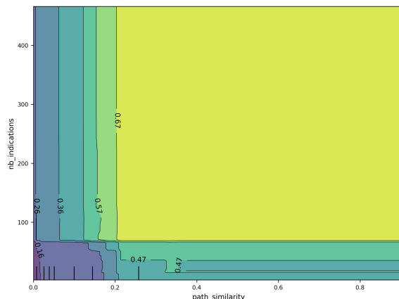
Figure 12: Two-dimensional partial dependence of the two most important features.
