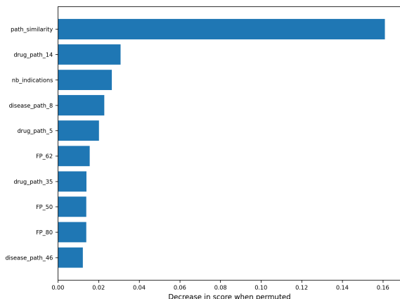
Figure 11: Permutation feature importance for trained XGBoost.
