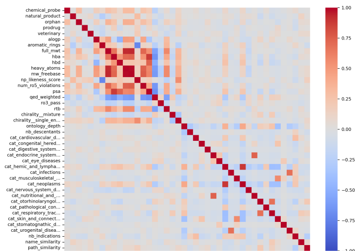
Figure 6: Focused view of the correlation heatmap on interpretable features.
