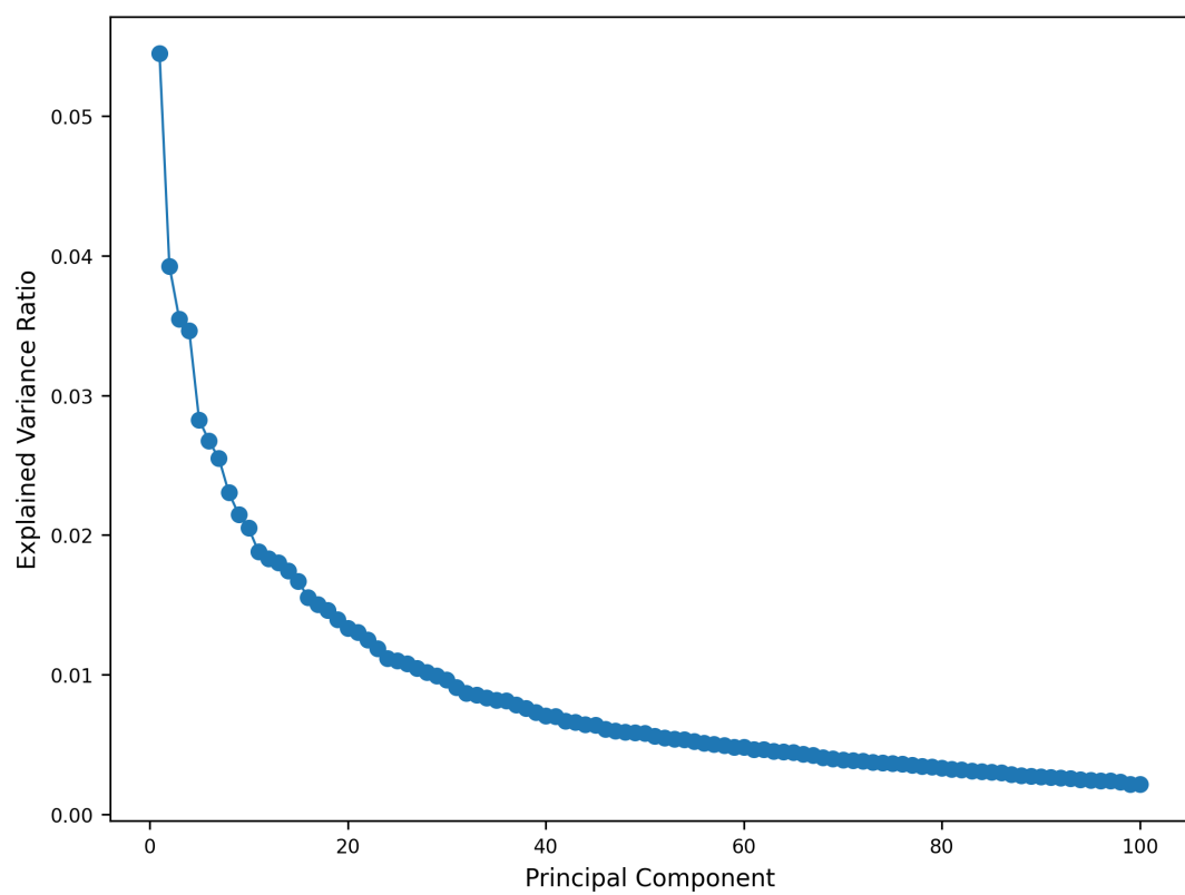
Figure A5: Scree plot of explained variance for PCA components.
