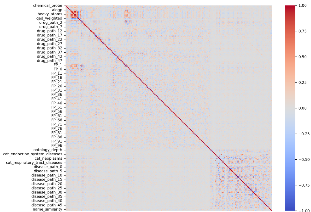
Figure A4: Correlation heatmap of all features.
