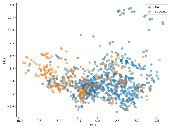
Figure 7: PCA projection of samples onto the first two principal components.
