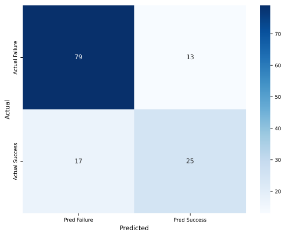
Figure 9: Confusion matrix for XGBoost on the test dataset.
