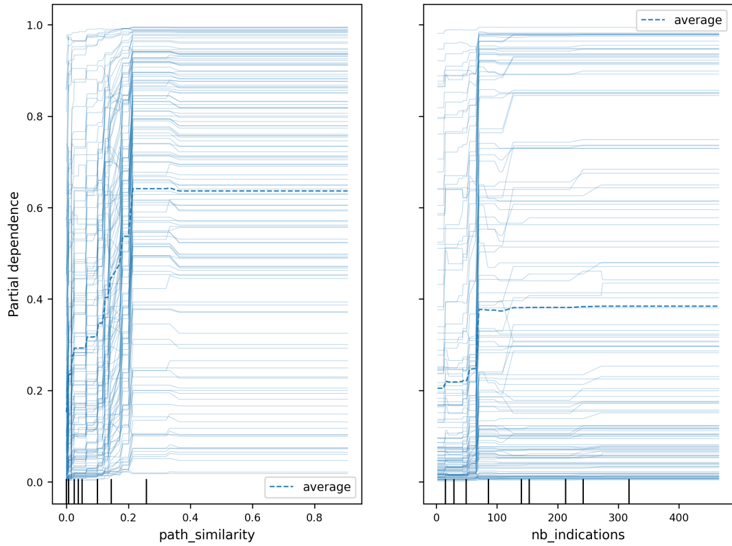
Figure A14: Partial dependence of the two most important features.
