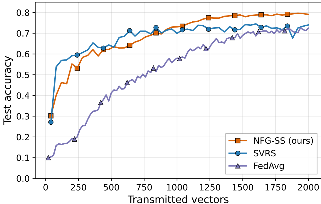
CIFAR-10, ResNet-18, n = 11 nodes
