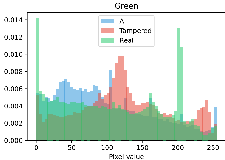
RGB Channel Distributions (pixel samples)
