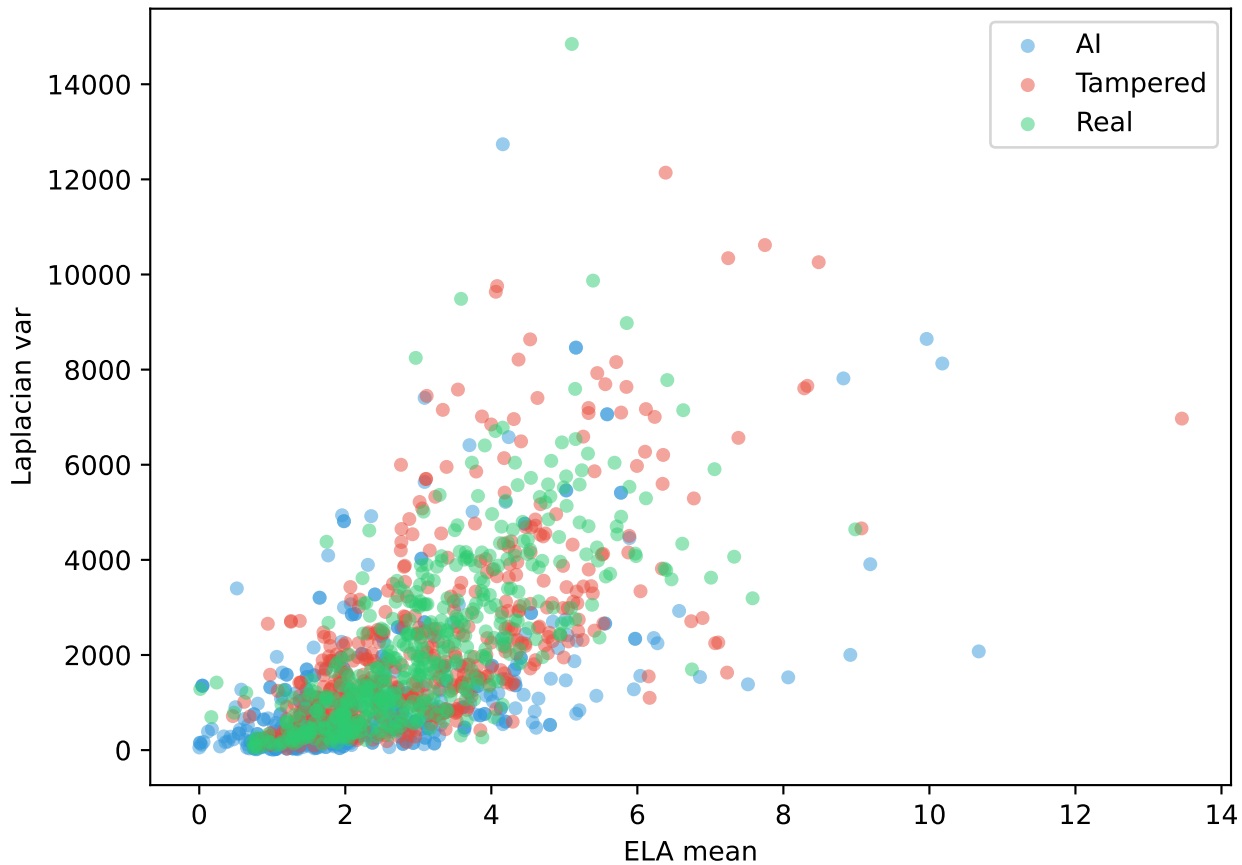
ELA mean vs Laplacian variance
