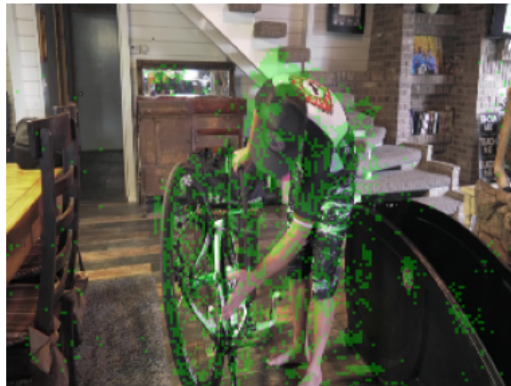
Prediction
