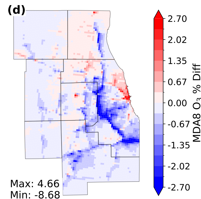
% Difference from Default
