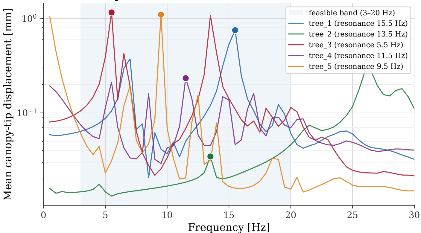
FRF sweeps across 5 trees — markers at in-band resonance
