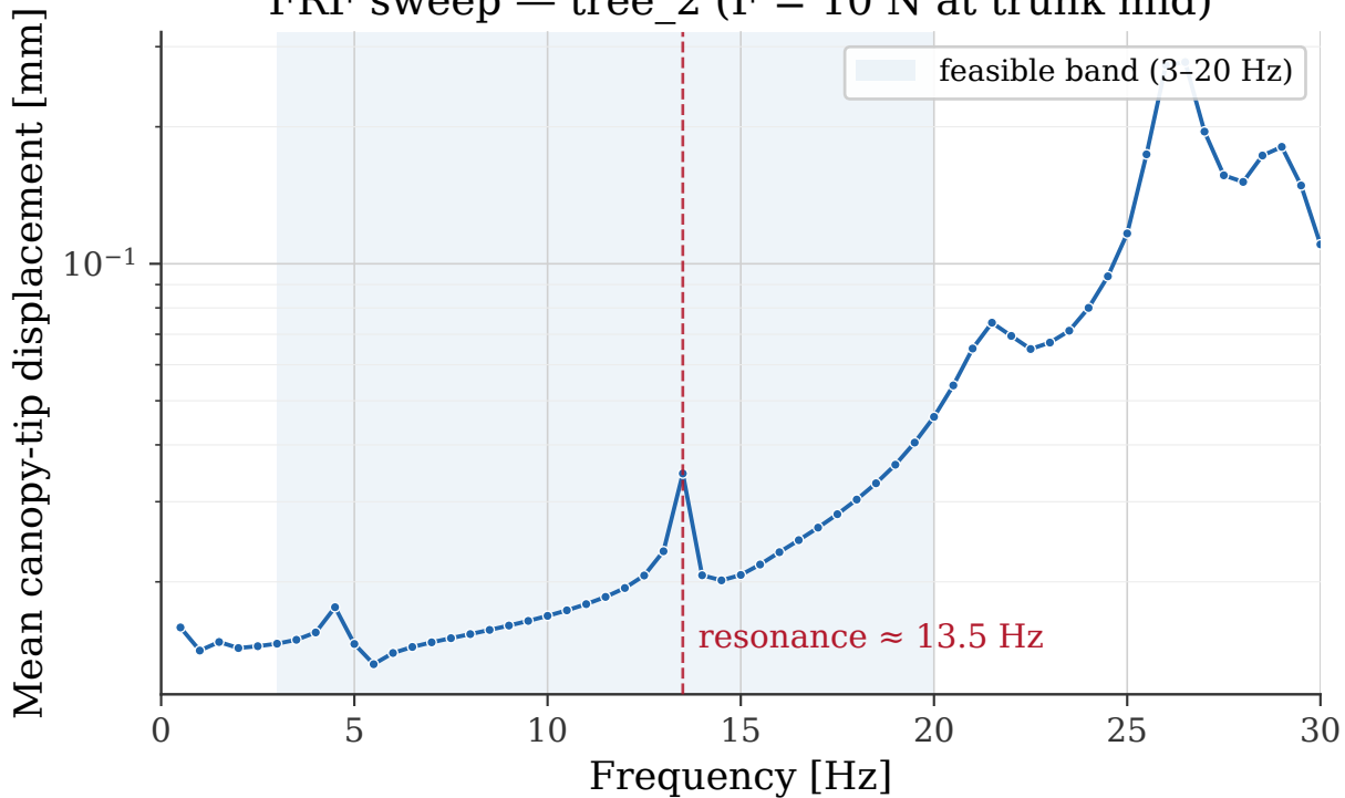
FRF sweep — tree_2 (F = 10 N at trunk mid)
