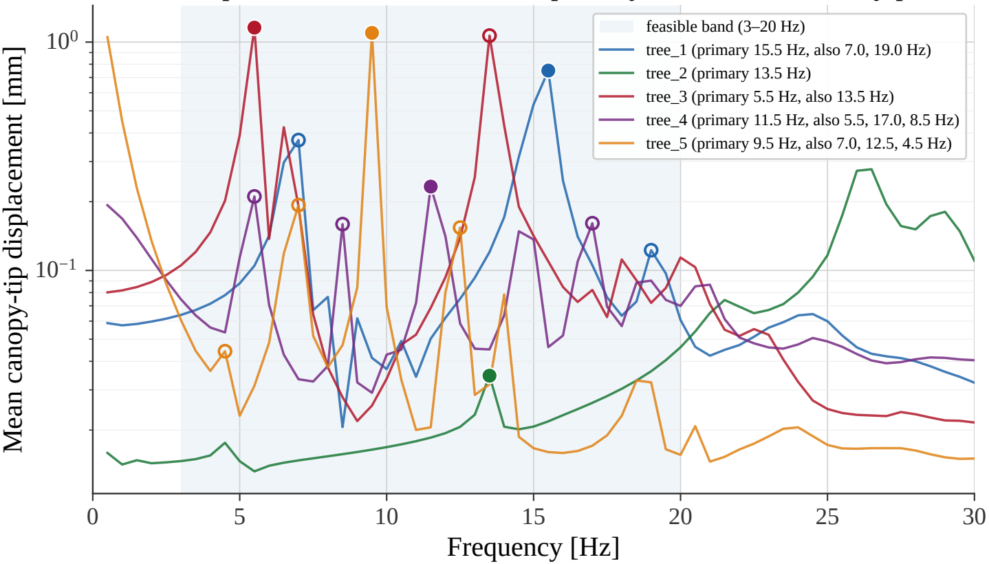
FRF sweeps across 5 trees — filled = primary, hollow = secondary peaks
