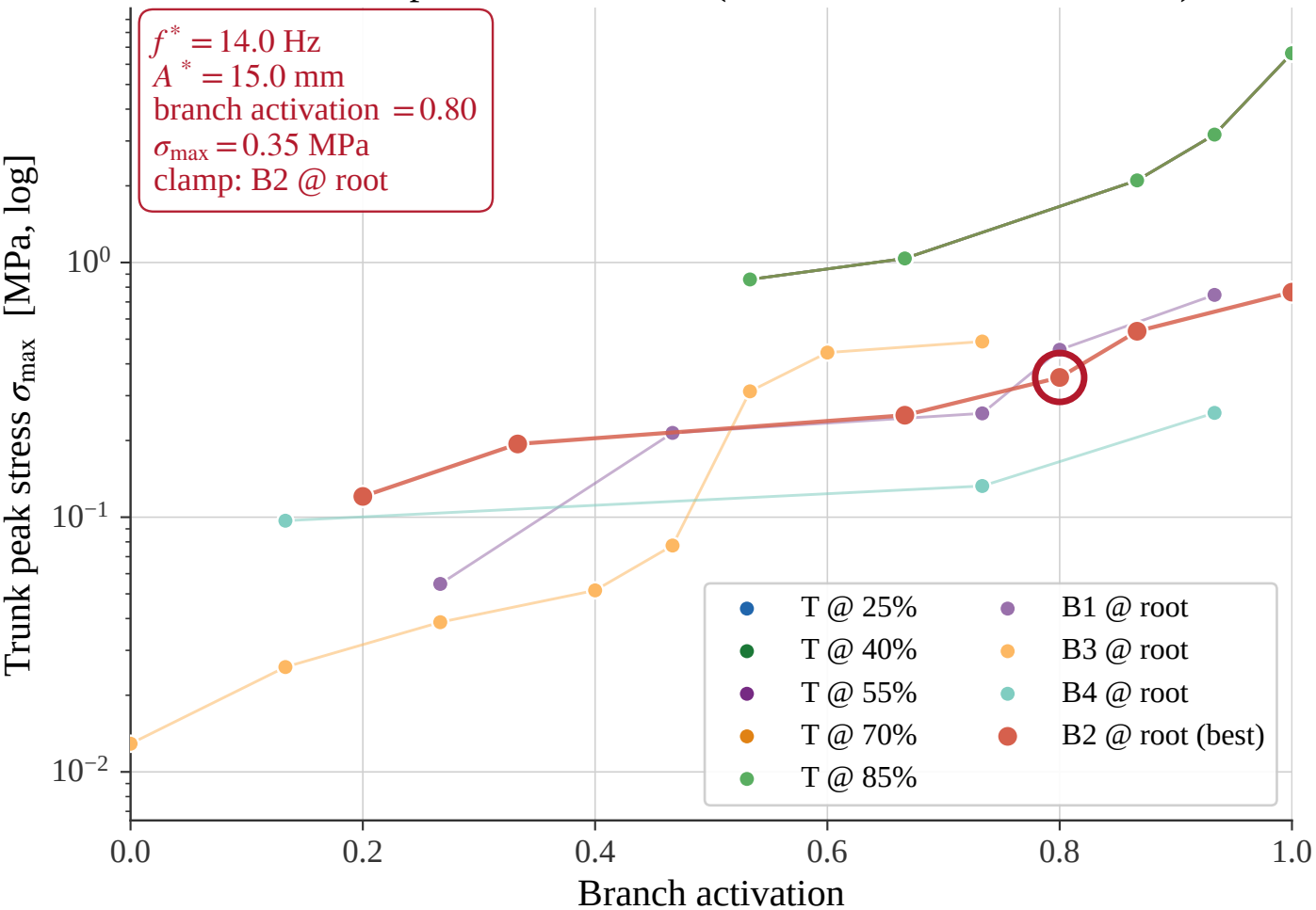
Multi-clamp Pareto — tree_2 (300 fruits, resonance 6.5 Hz)
