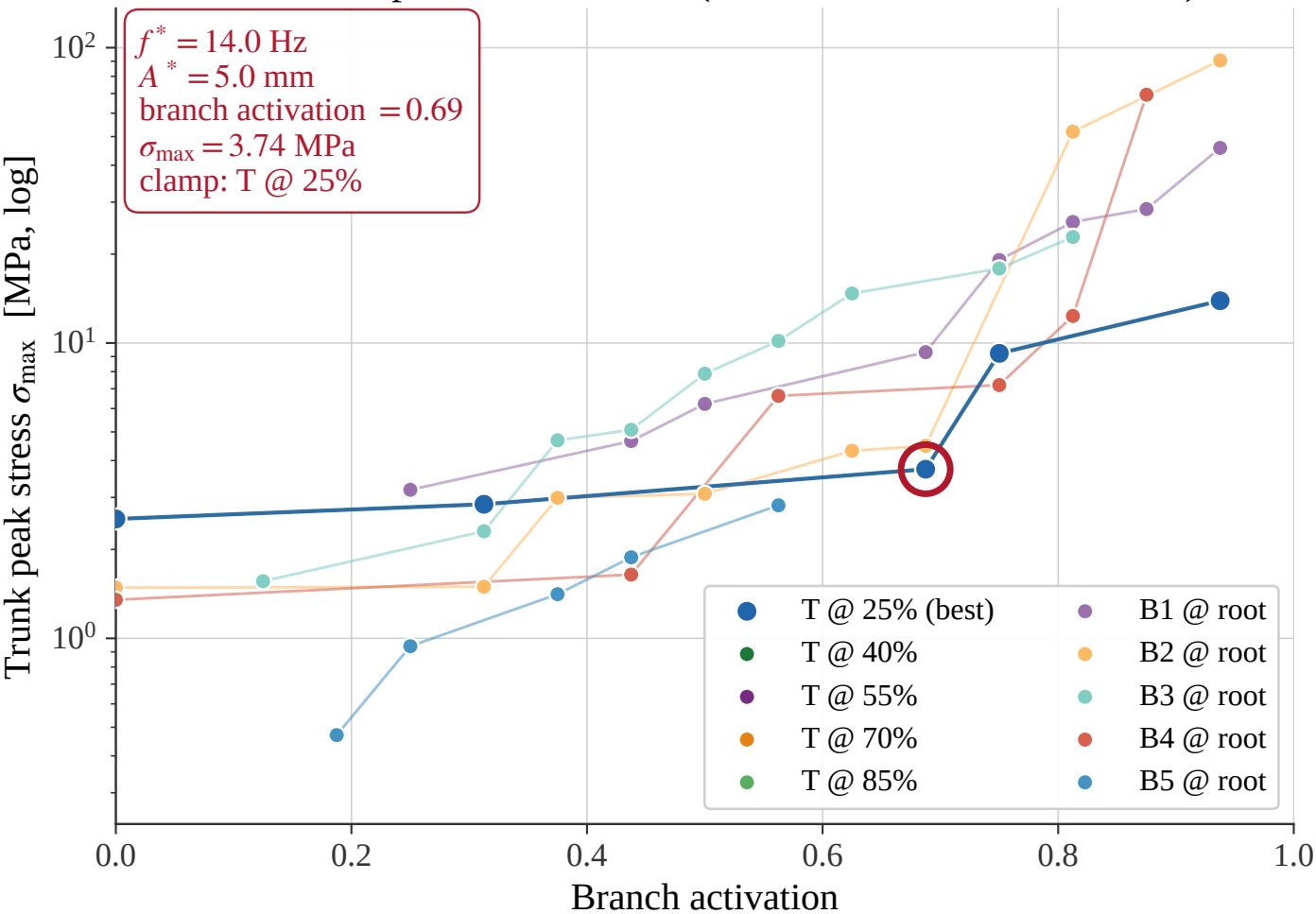
Multi-clamp Pareto — tree_4 (320 fruits, resonance 12.0 Hz)
