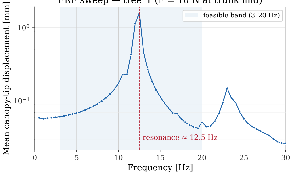
FRF sweep — tree_1 (F = 10 N at trunk mid)
