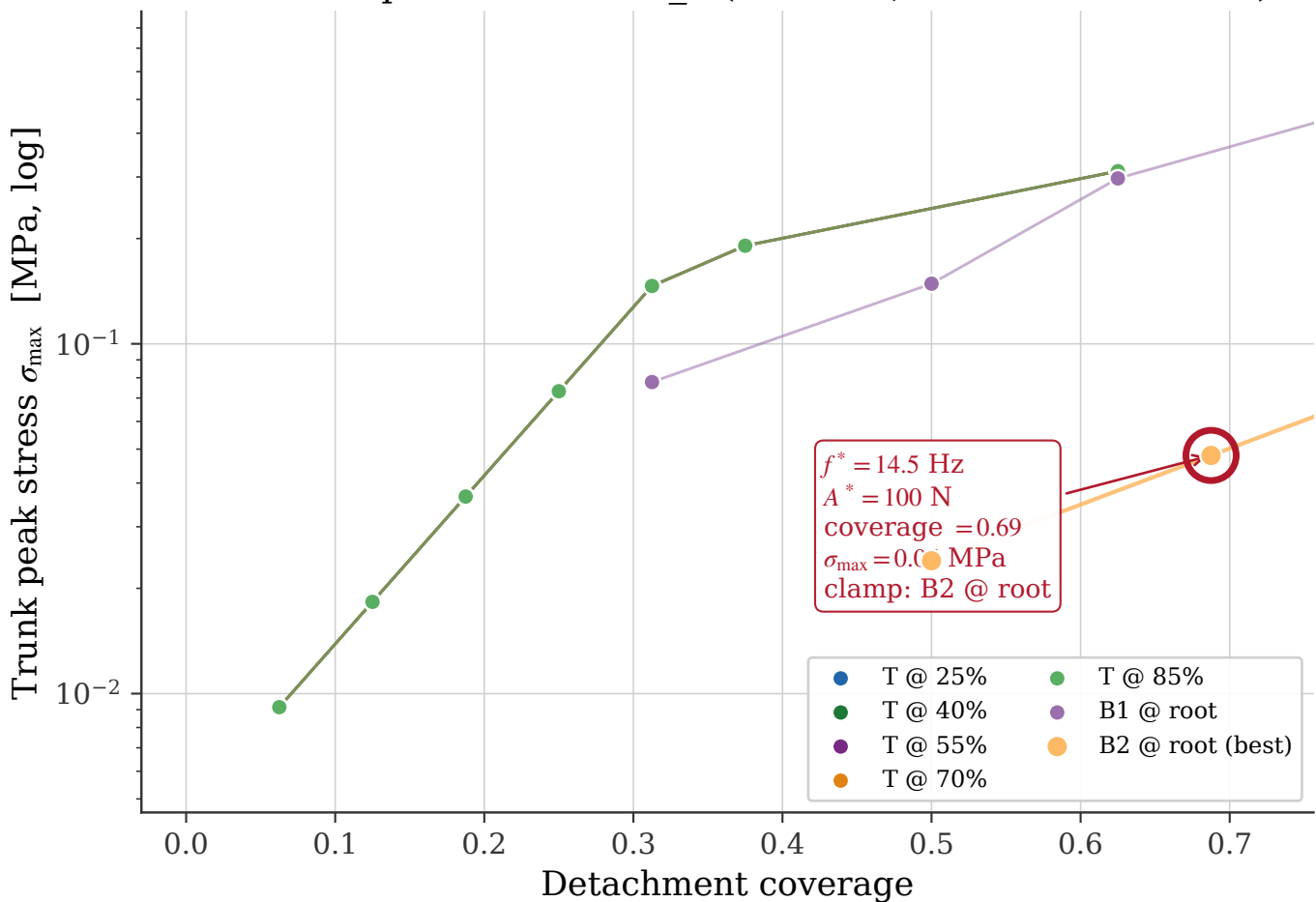
Multi-clamp Pareto — tree_1 (16 fruits, resonance 12.5 Hz)
