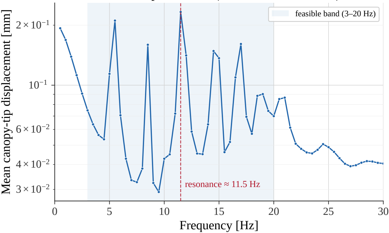
FRF sweep — tree_4 (F = 10 N at trunk mid)
