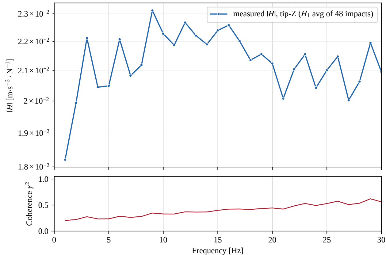
Measured FRF — tip station, vertical (Z)
