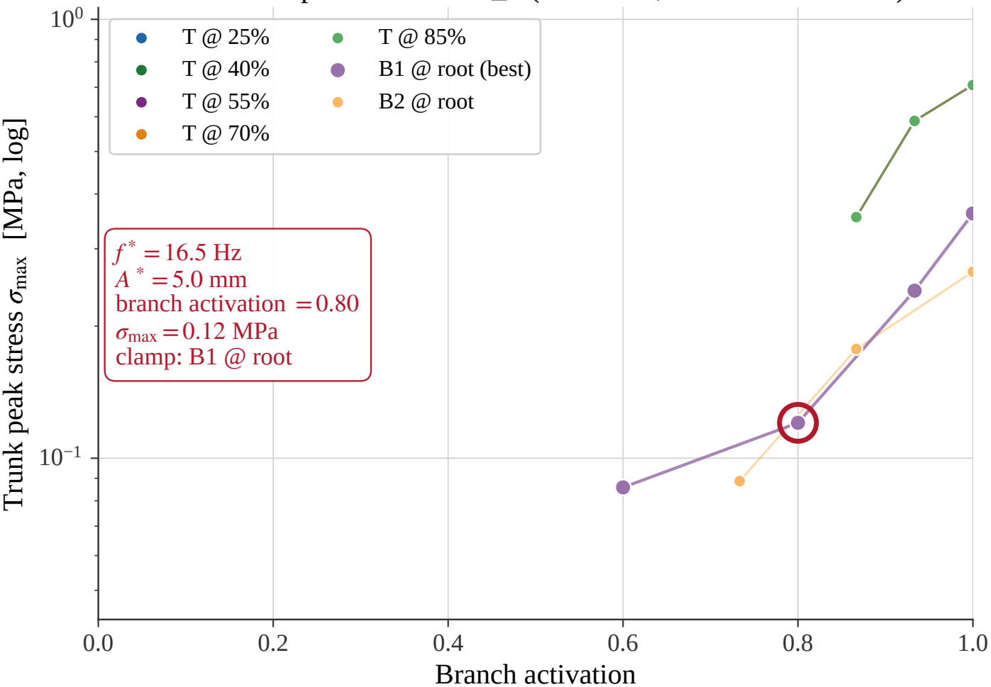
Multi-clamp Pareto — tree_1 (300 fruits, resonance 15.5 Hz)
