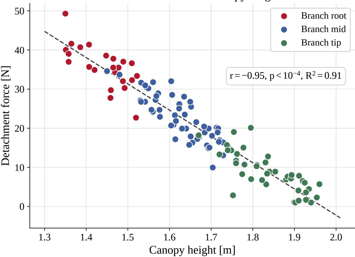
Detachment force vs. canopy height
