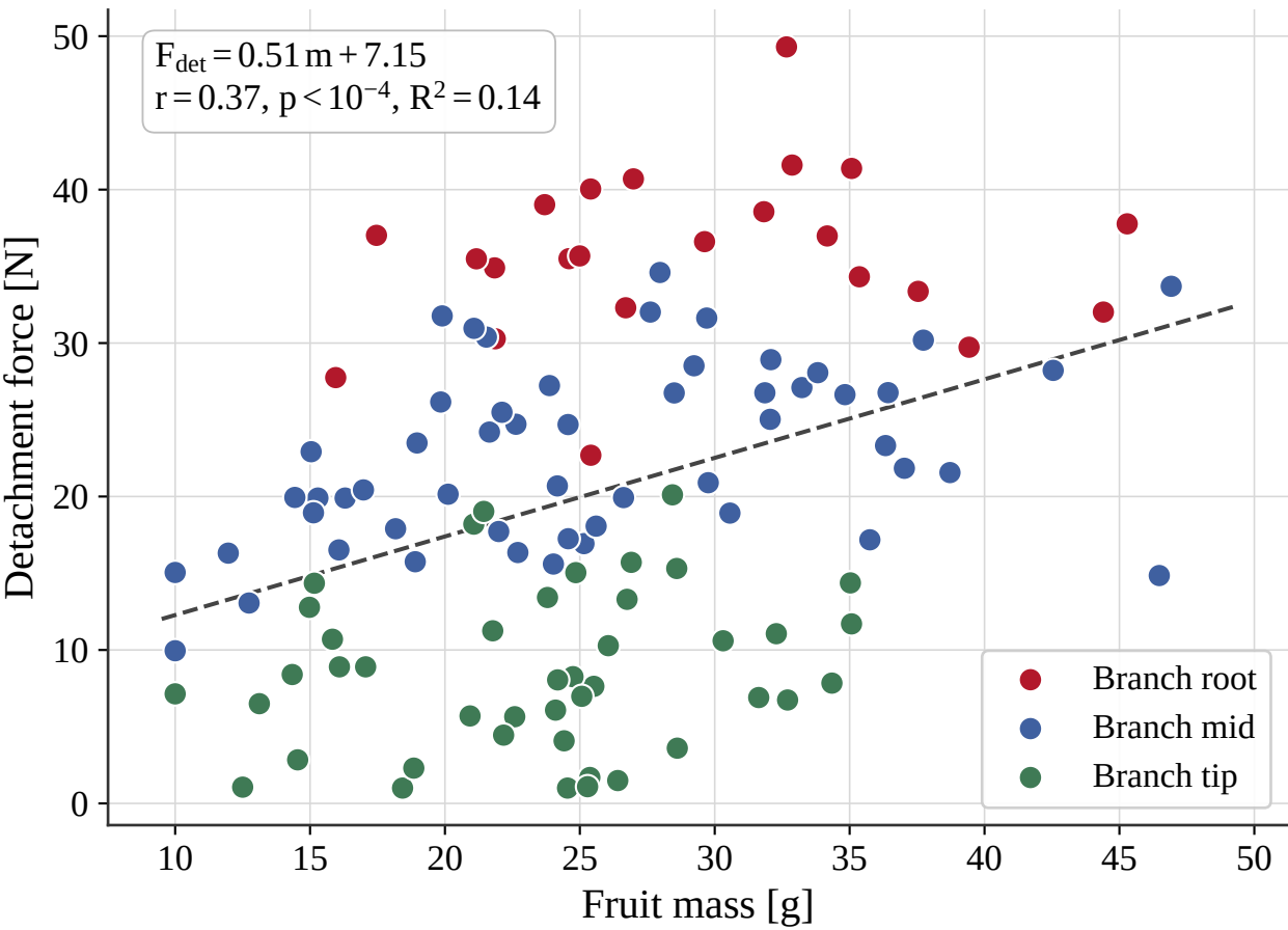
Detachment force vs. fruit mass
