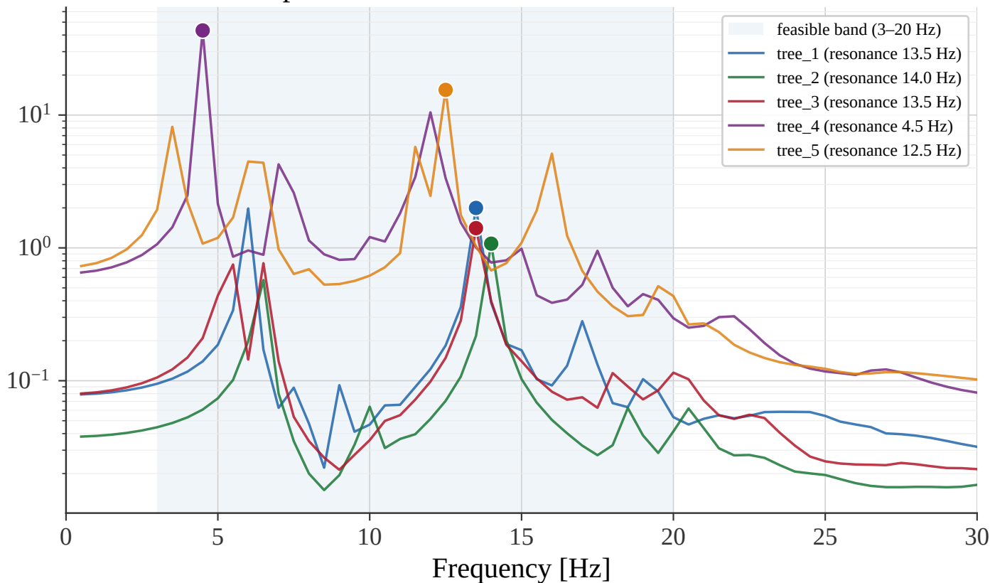
FRF sweeps across 5 trees — markers at in-band resonance
