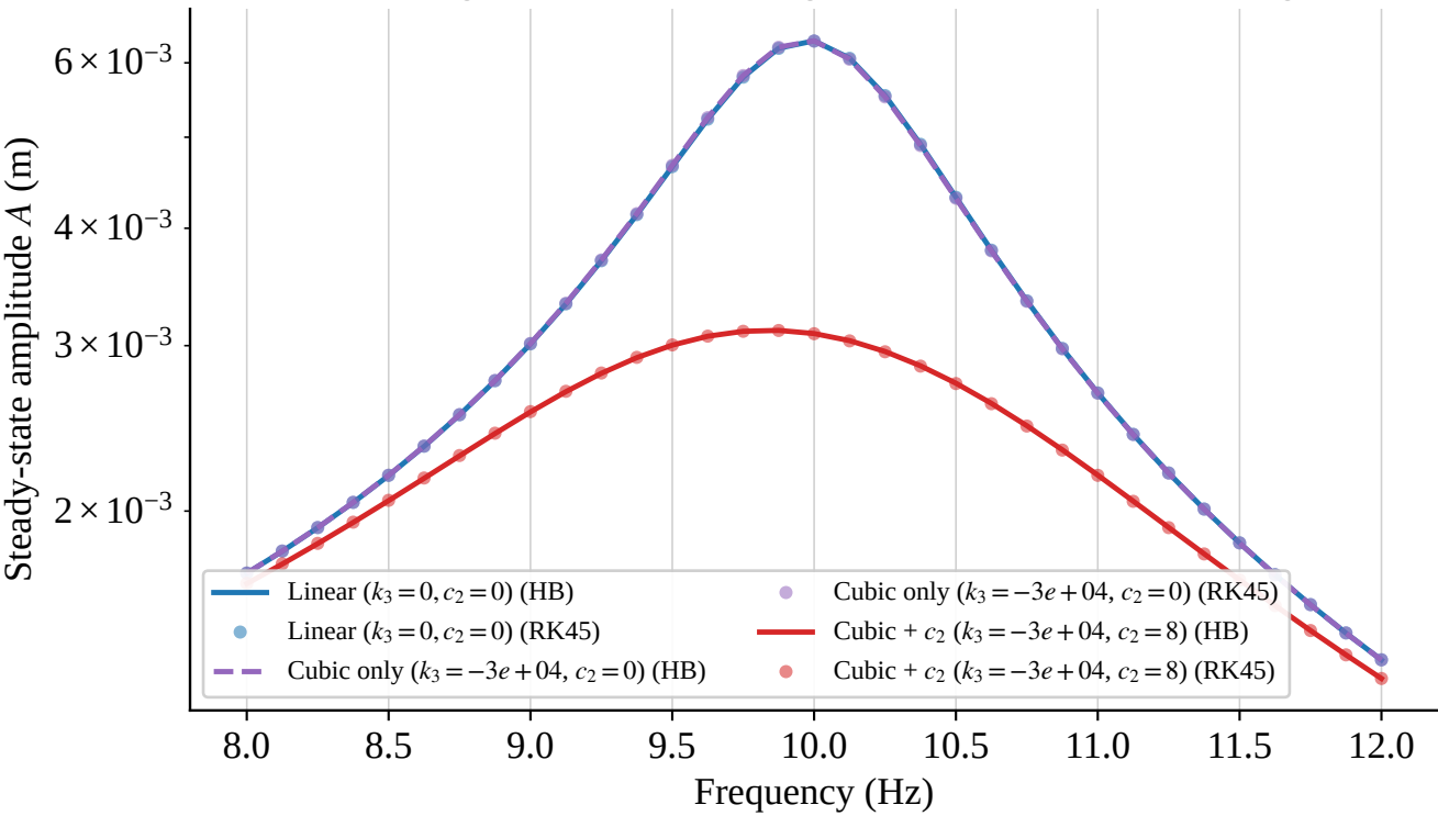
SDOF Duffing FRF: HB describing function vs RK45 time integration
