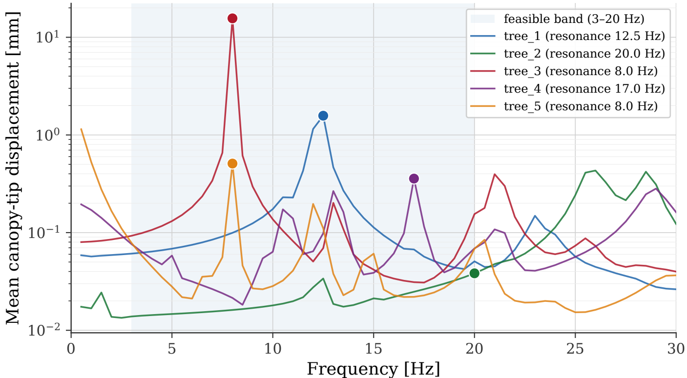
FRF sweeps across 5 trees — markers indicate in-band resonance
