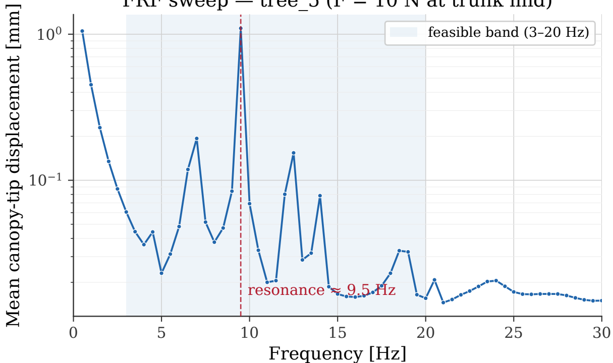
FRF sweep — tree_5 (F = 10 N at trunk mid)
