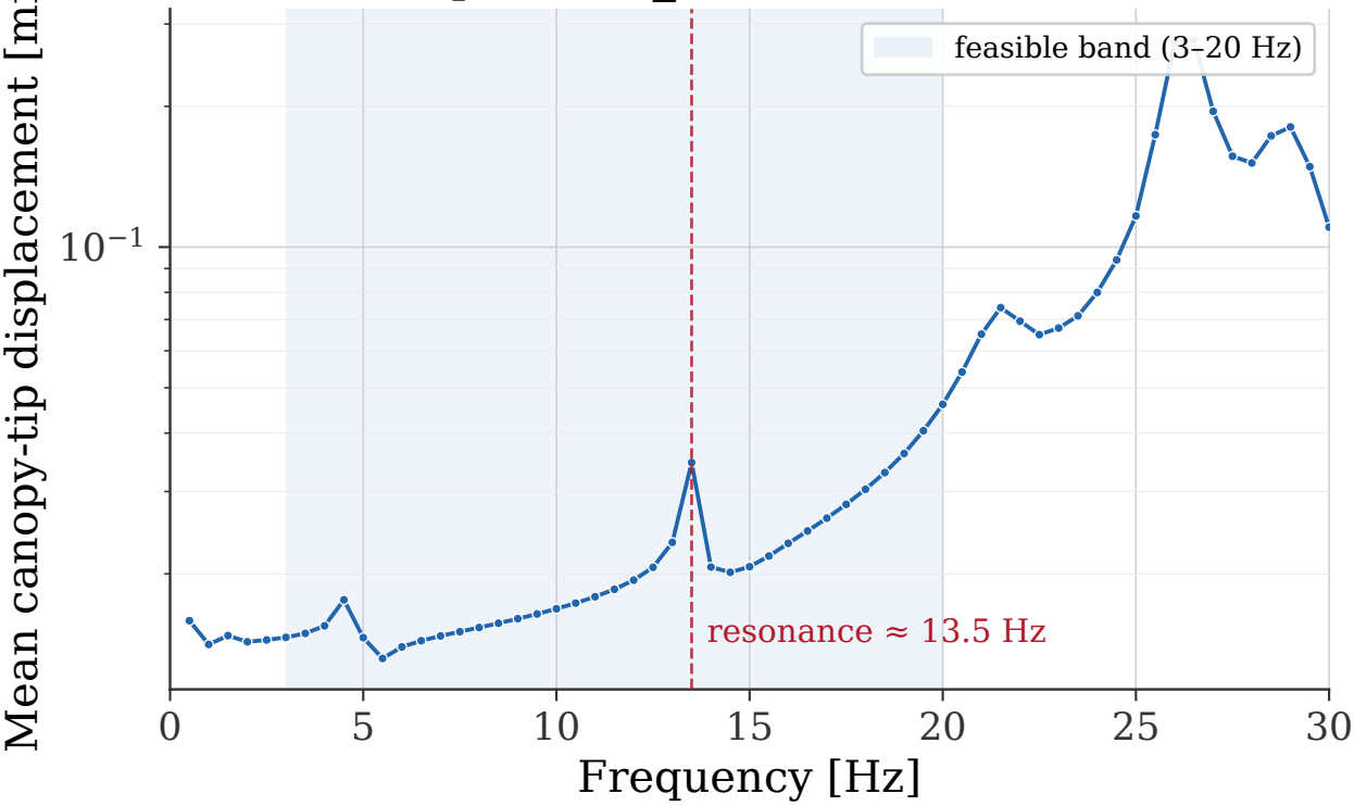
FRF sweep — tree_2 ( F = 10\text{ N} at trunk mid)
