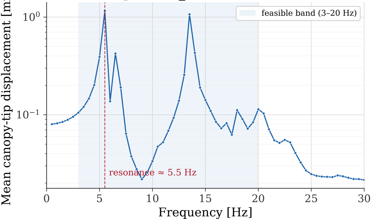
FRF sweep — tree_3 (F = 10 N at trunk mid)
