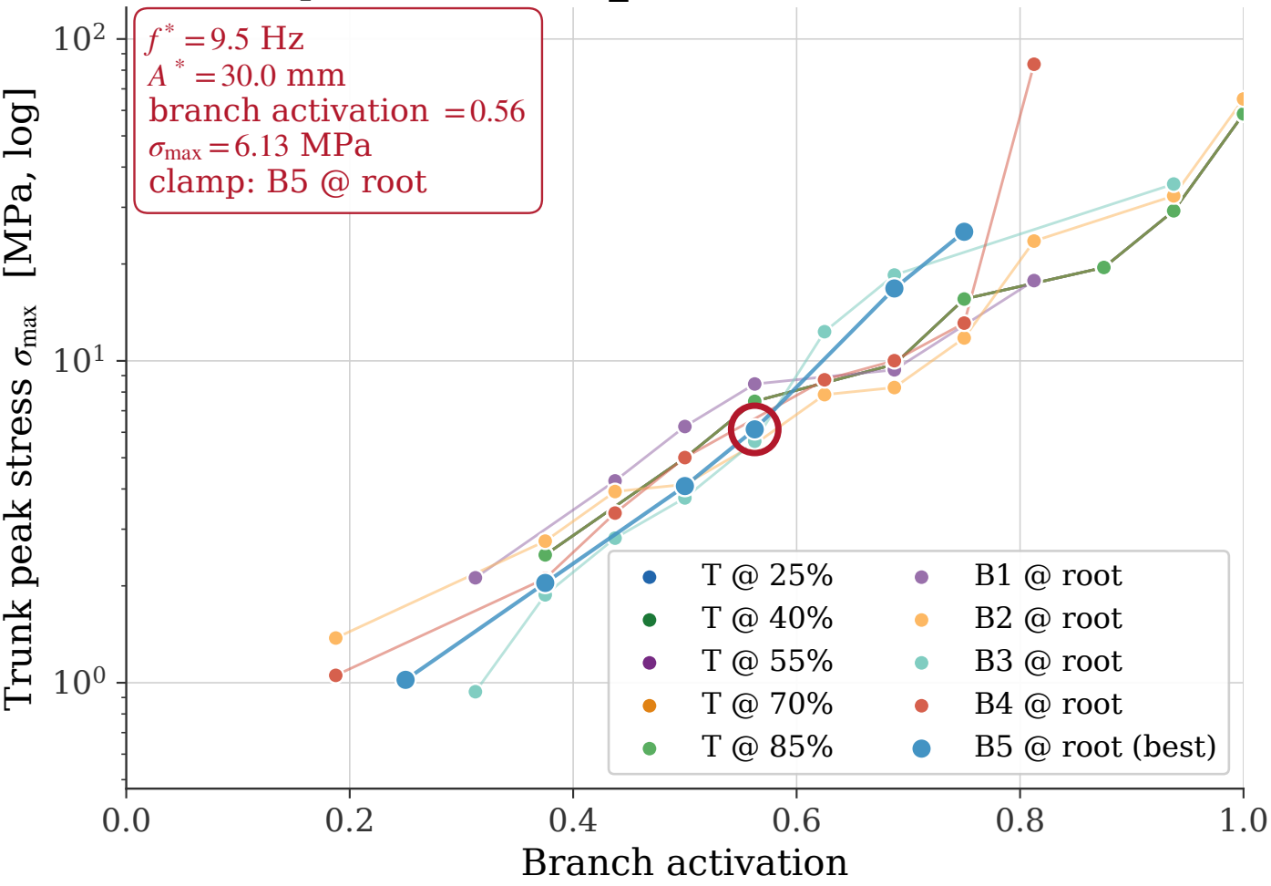
Multi-clamp Pareto — tree 4 (320 fruits, resonance 11.5 Hz)
