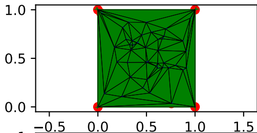
Original Graph
