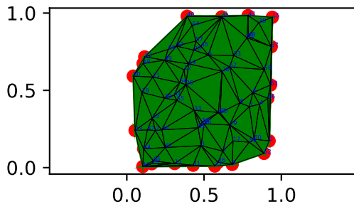
Original Graph
