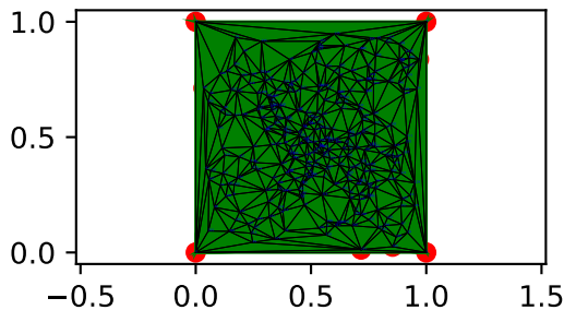
Original Graph
