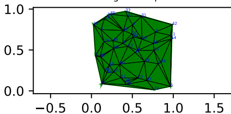
Original Graph
