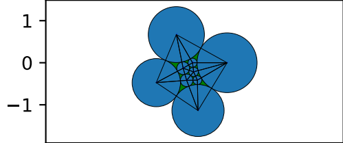
-2 AES minimized graph 2
