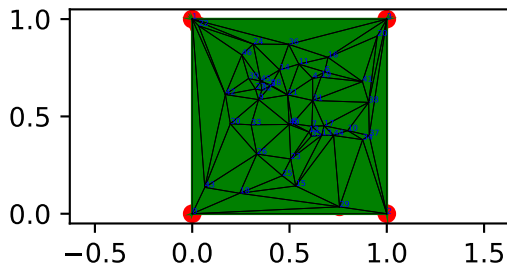
Original Graph
