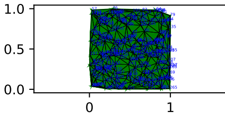
Original Graph
