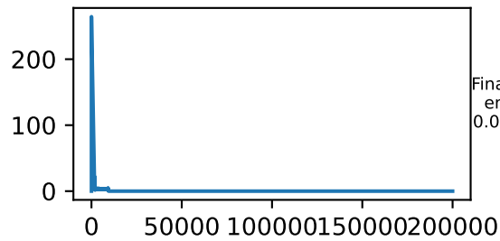
Second Constraint Energy
