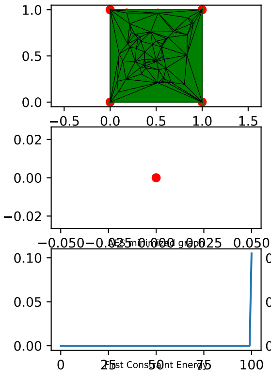
Original Graph
