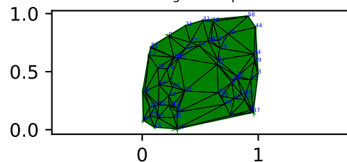
Original Graph
