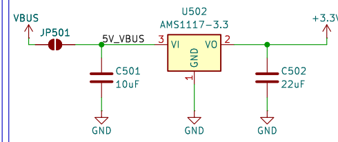
VBus to 3.3V circuitry
