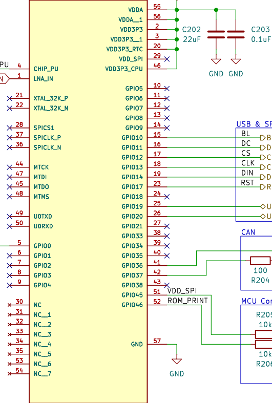
U201 ESP32-S3-PICO-1-N8R2
