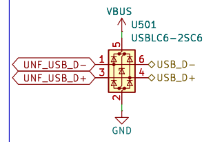
Surge Protection
