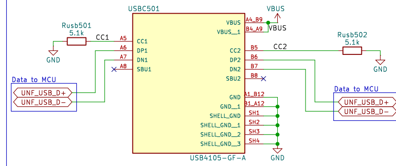
USB-C Port
