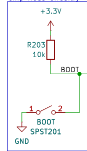
Chip Mode Circuitry
