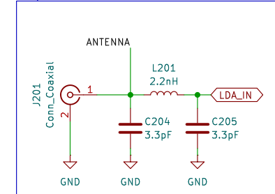
WiFi/Bluetooth Antenna
