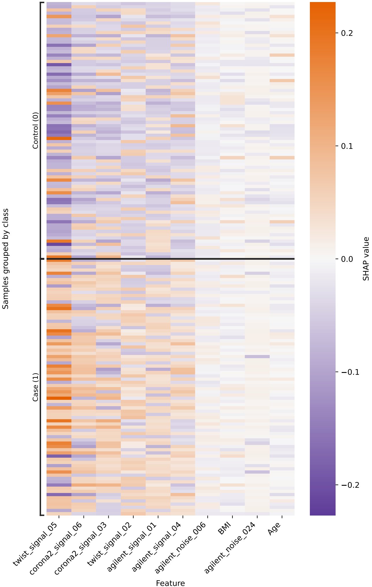
Signed SHAP values across samples
