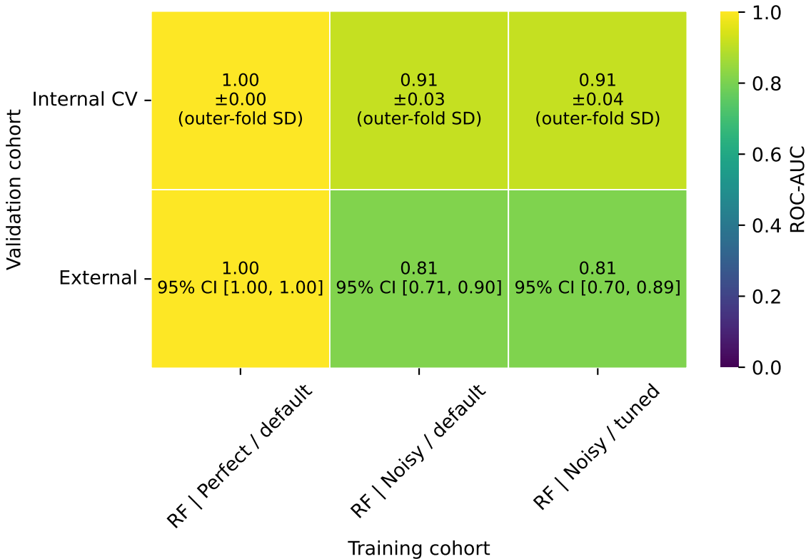
random-forest: internal CV and external ROC-AUC
