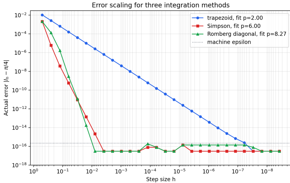
图 3: Problem 3 error scaling
