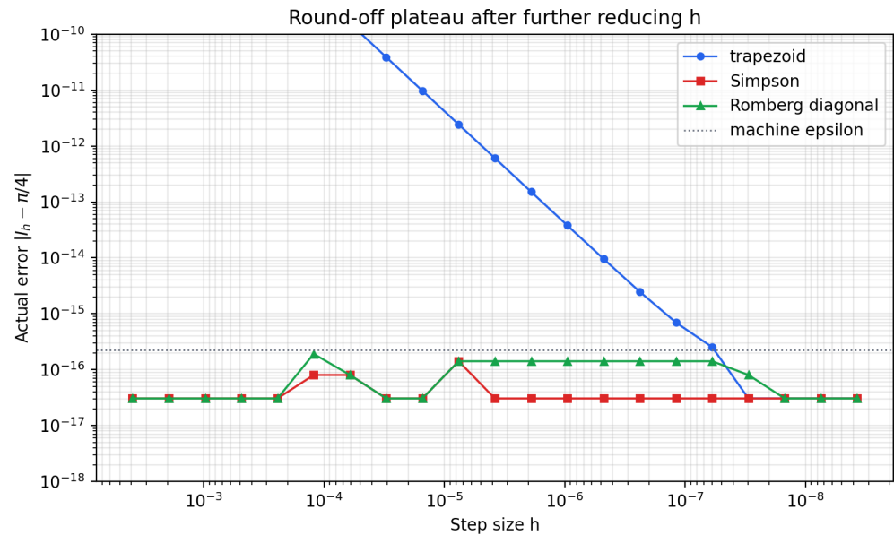
图 4: Problem 3 round-off zoom
