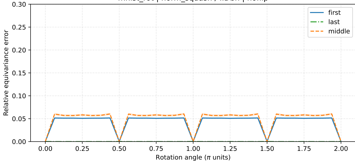
mnist_rot | norm_squash / IIDbn | noflip
