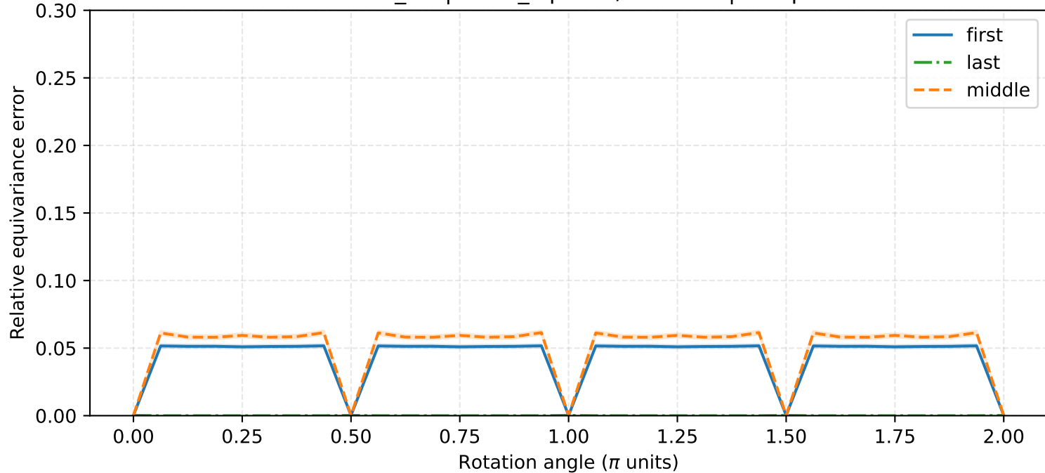
mnist_rot | norm_squash / Normbn | noflip
