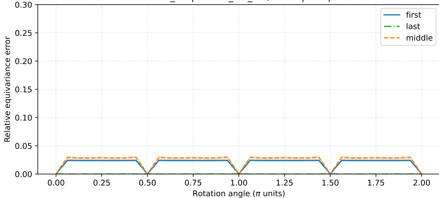
mnist_rot | fourier_elu_32 / IIDbn | noflip
