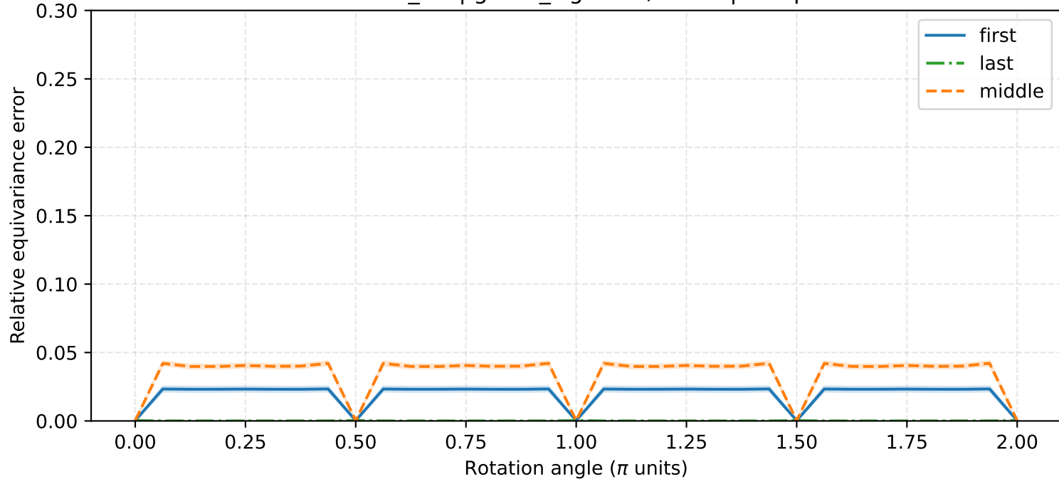
mnist_rot | gated_sigmoid / IIDbn | noflip
