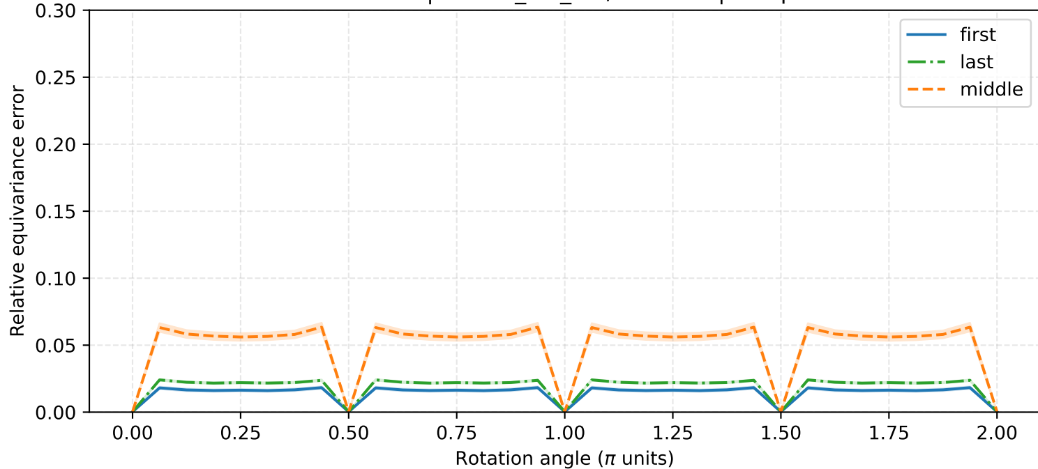
eurosat | fourier_elu_32 / Normbn | noflip
