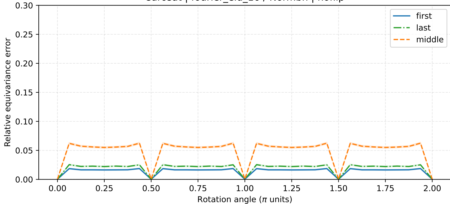
eurosat | fourier_elu_16 / Normbn | noflip
