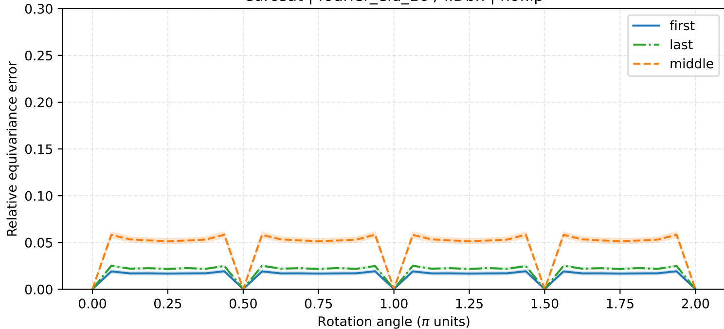
eurosat | fourier_elu_16 / IIDbn | noflip
