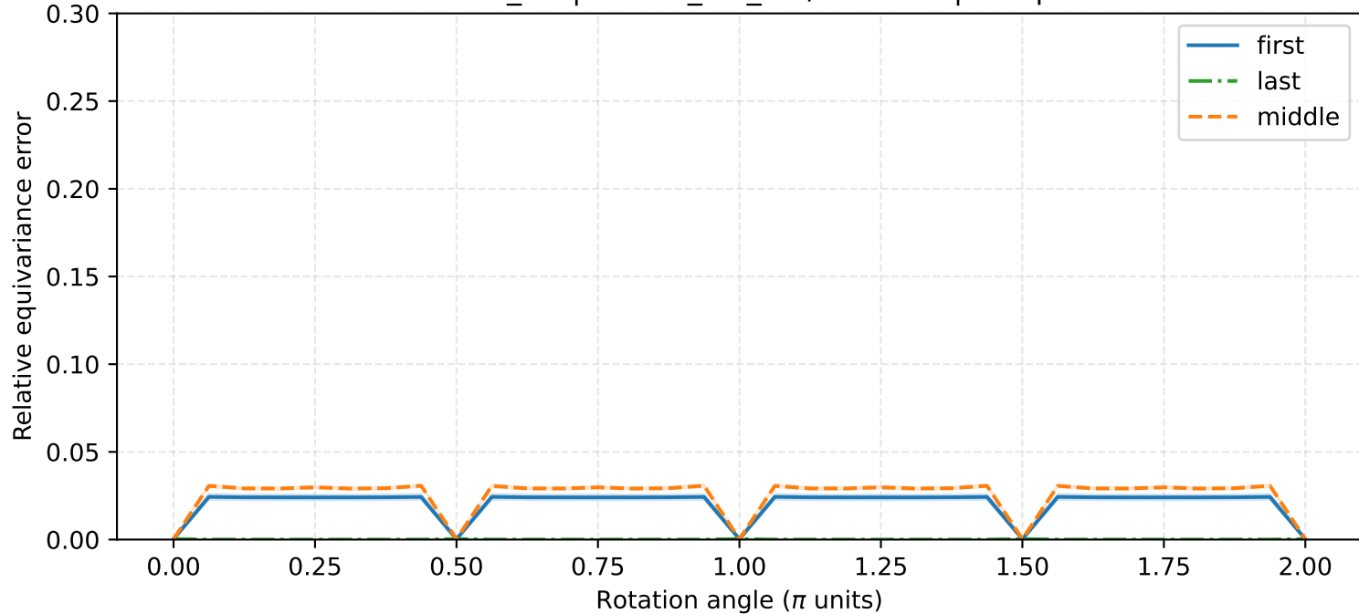
mnist_rot | fourier_elu_32 / Normbn | noflip
