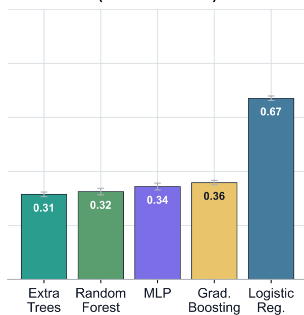
Ordinal MAE (lower is better)
